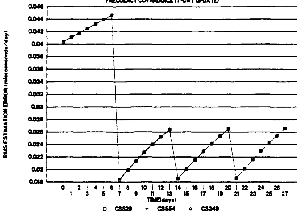
Figure 3.1-4e Frequency Covariance (7 Day Update)
