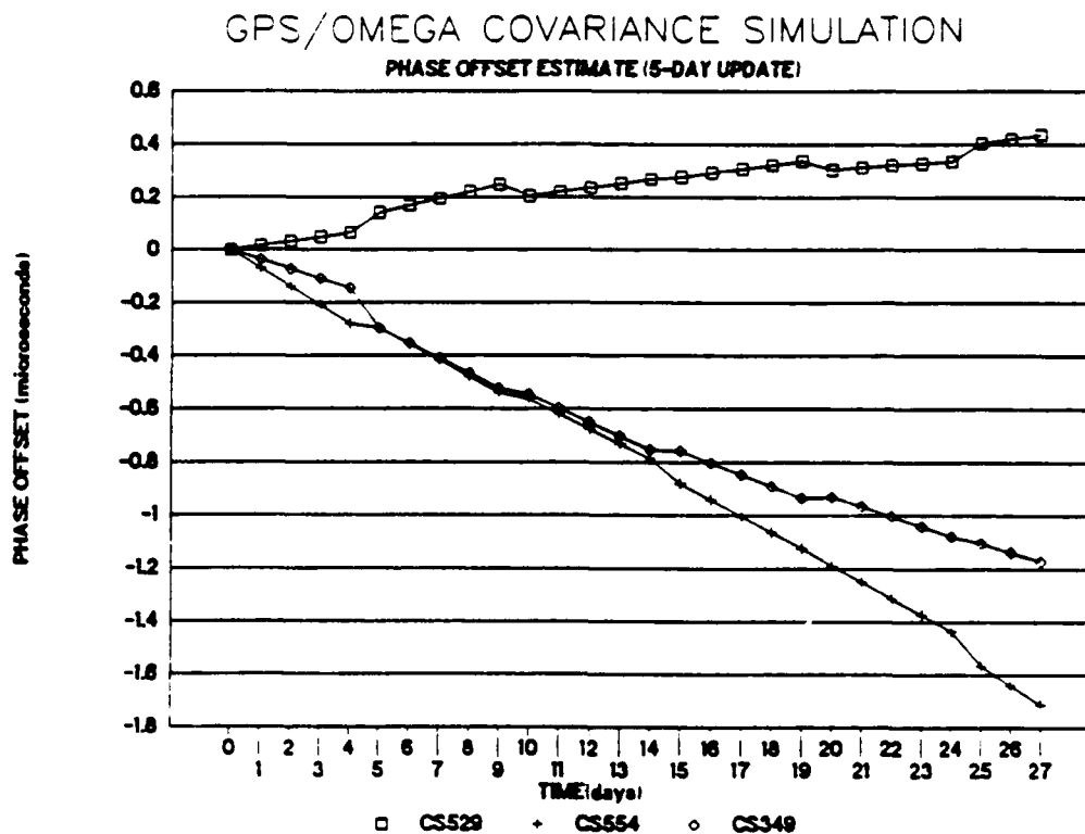
Figure 3.4-3a Phase Offset Estimate (5 Day Update)
