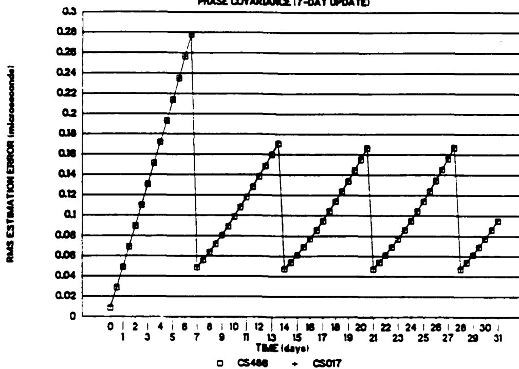
Figure 2.3-4c Phase Covariance (7 Day Update)
