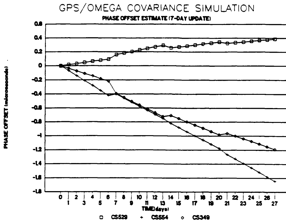
Figure 3.4-4a Phase Offset Estimate (7 Day Update)
