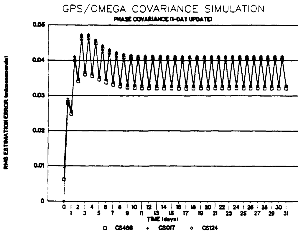
Figure 2.2-1c Phase Covariance (1 Day Update)
