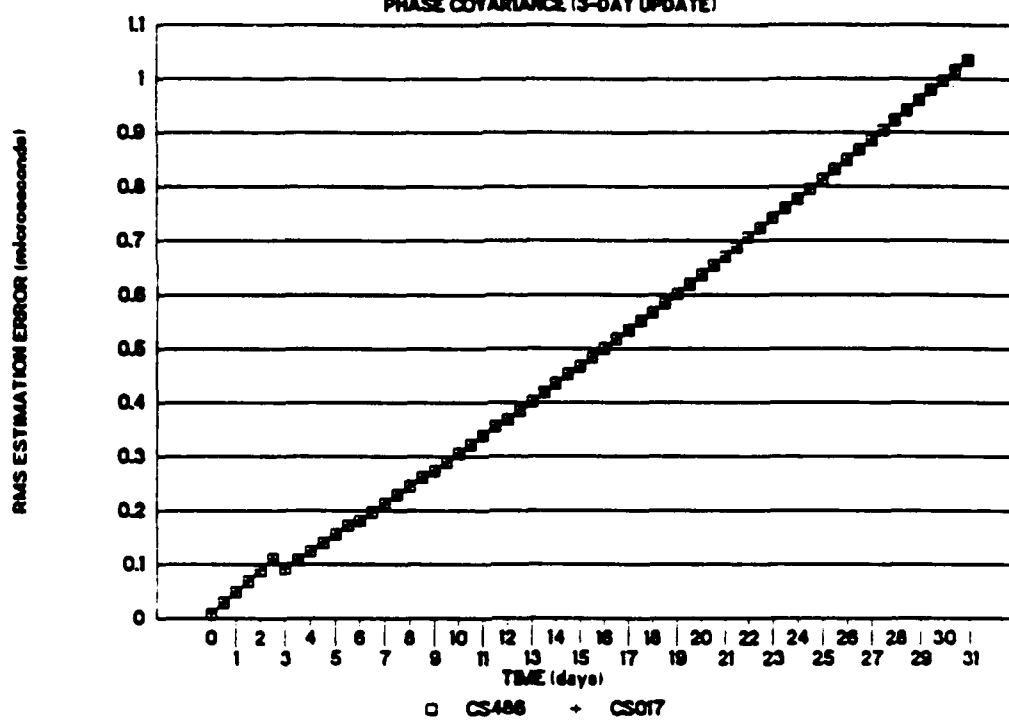
Figure 2.5-2c Phase Covariance (3 Day Update)
