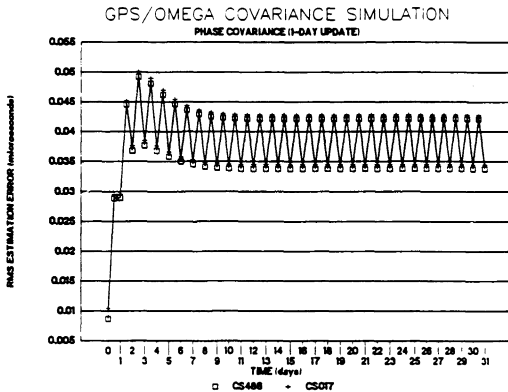
Figure 2.3-1c Phase Covariance (1 Day Update)
