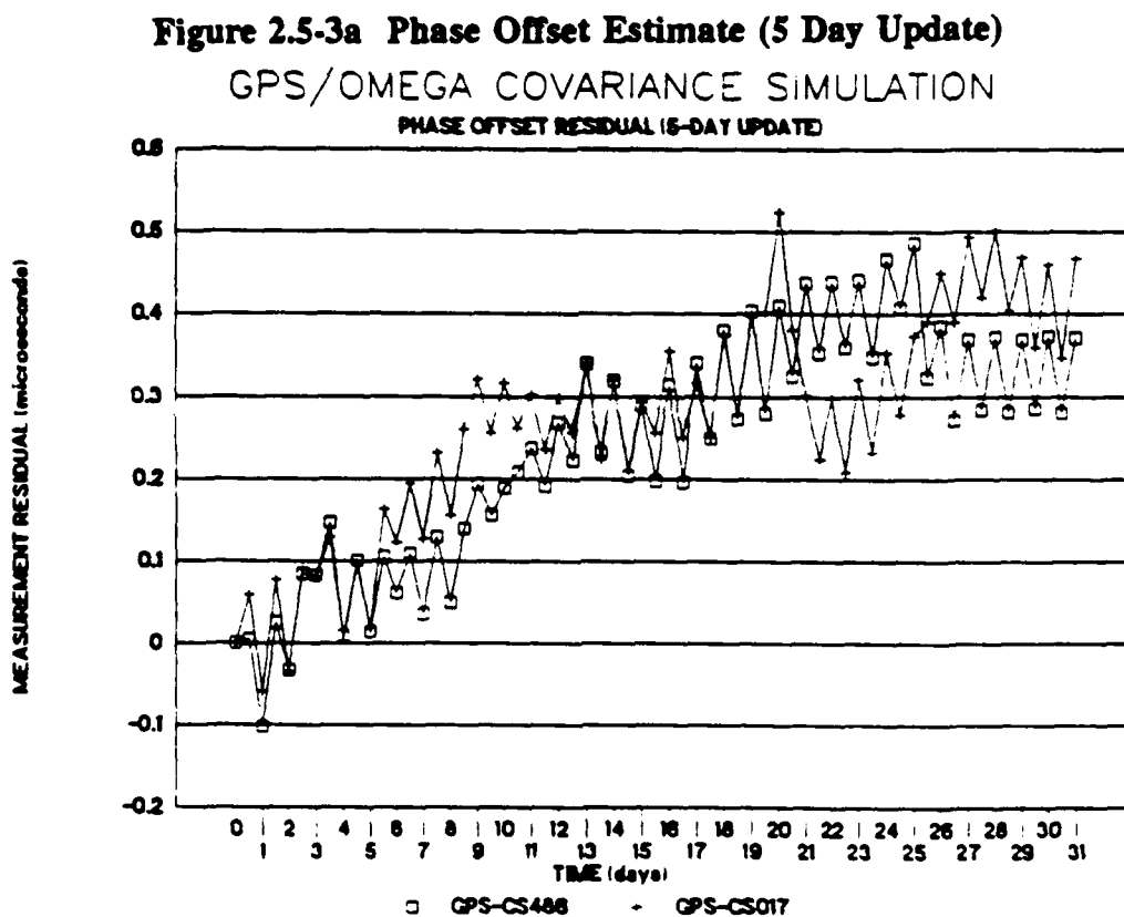
Figure 2.5-3b Phase Offset Residual: GPS-CS486, GPS-CS017 (5 Day Update)
