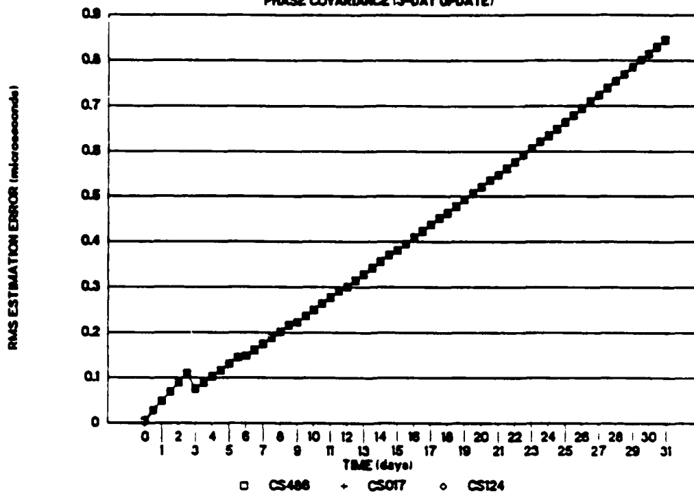
Figure 2.4-2c Phase Covariance (3 Day Update)
