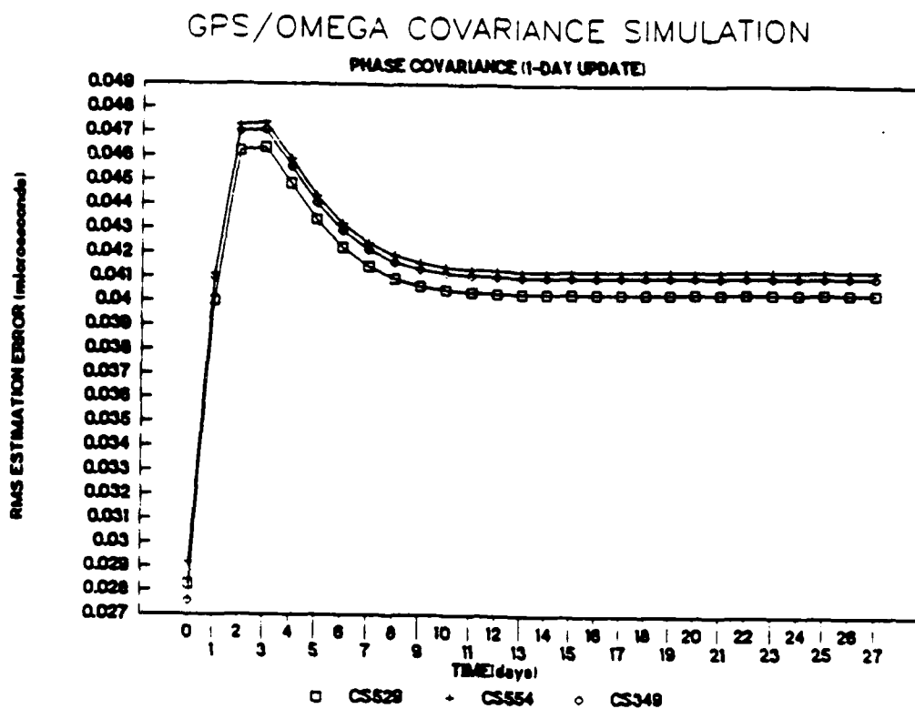
Figure 3.2-1c Phase Covariance (1 Day Update)
