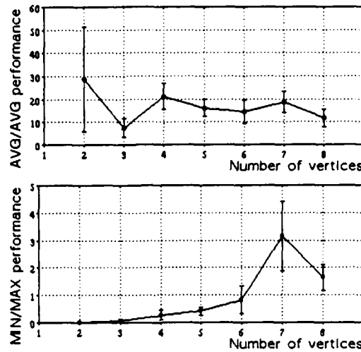
Figure 12: AVG/AVG and MIN/MAX indices vs. the number of vertices used in training (the data for number of vertices from 2 to 6 are for six-vertex random wire objects; the data for number of vertices 7 and 8 are for eight-vertex wires; M = K = 60 , \sigma = 30.0 ).
