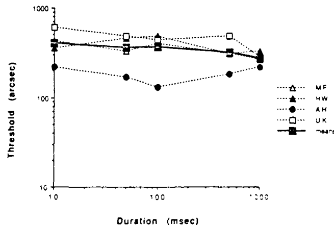
Fig. 3 Displacement thresholds in a bisection experiment. Conditions were similar to those for Fig. 2, but only the lower segment of the vernier was presented. The task was to indicate whether this segment was nearer to the left or to the right border of the monitor. These thresholds give the displacement required for detection. As both segments were always displaced into opposite directions, but only one segment was actually shown here, absolute bisection thresholds would be lower by a factor of 2. These experiments, however, were intended to rule out bisection as a possible cue in the previous experiments. Therefore, thresholds were calculated in a way corresponding to the previous experiments.
