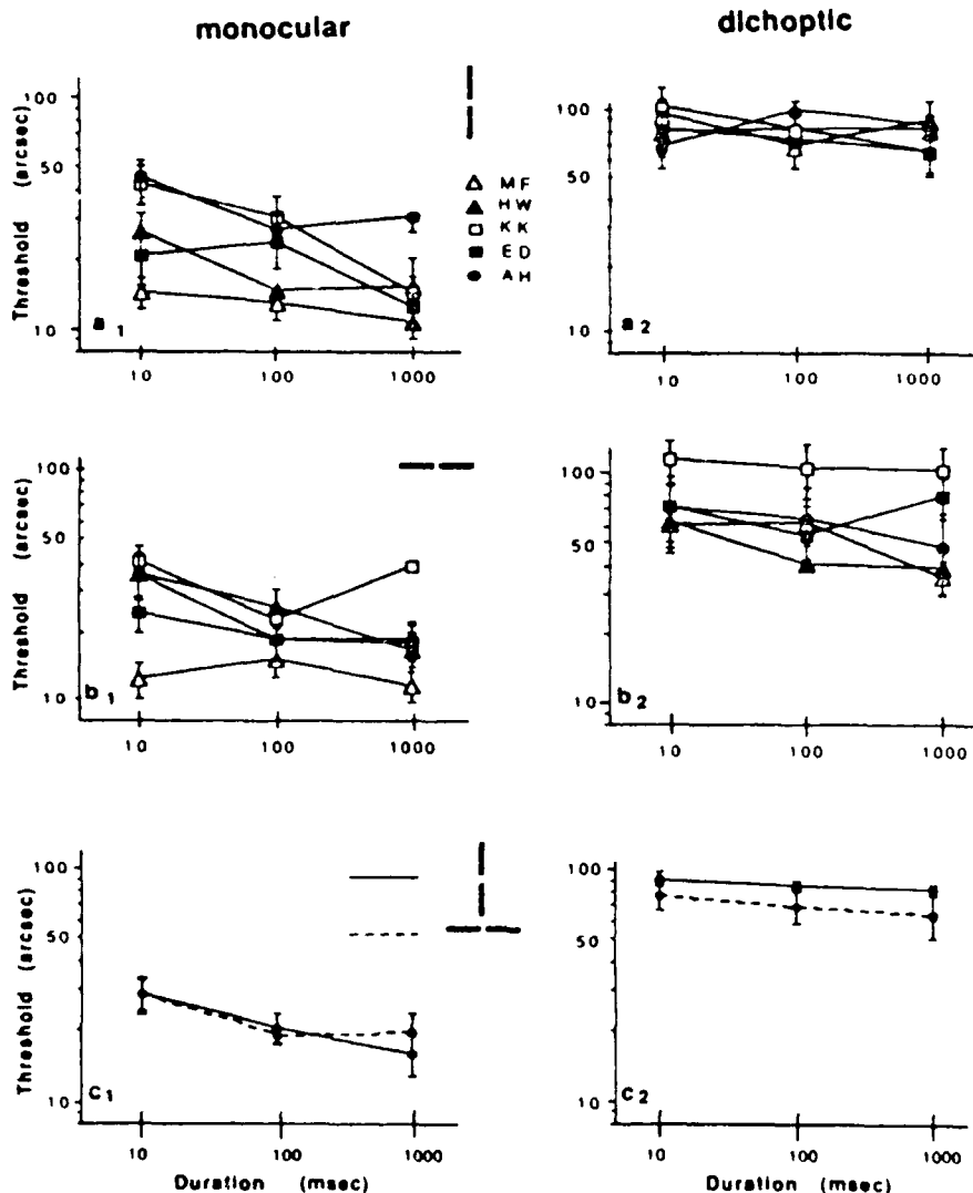
Fig. 1 Thresholds for vernier acuity with monocular presentation (left column) and with dichoptic presentation (right column) for five observers. The vernier target was presented for 10, 100 or 1000 msec (see abscissa). Fig. 1a shows results for vertical vernier targets, whereas Fig. 1b shows those for horizontal targets. Fig. 1c shows the means and standard errors of Figs. 1a and 1b.
