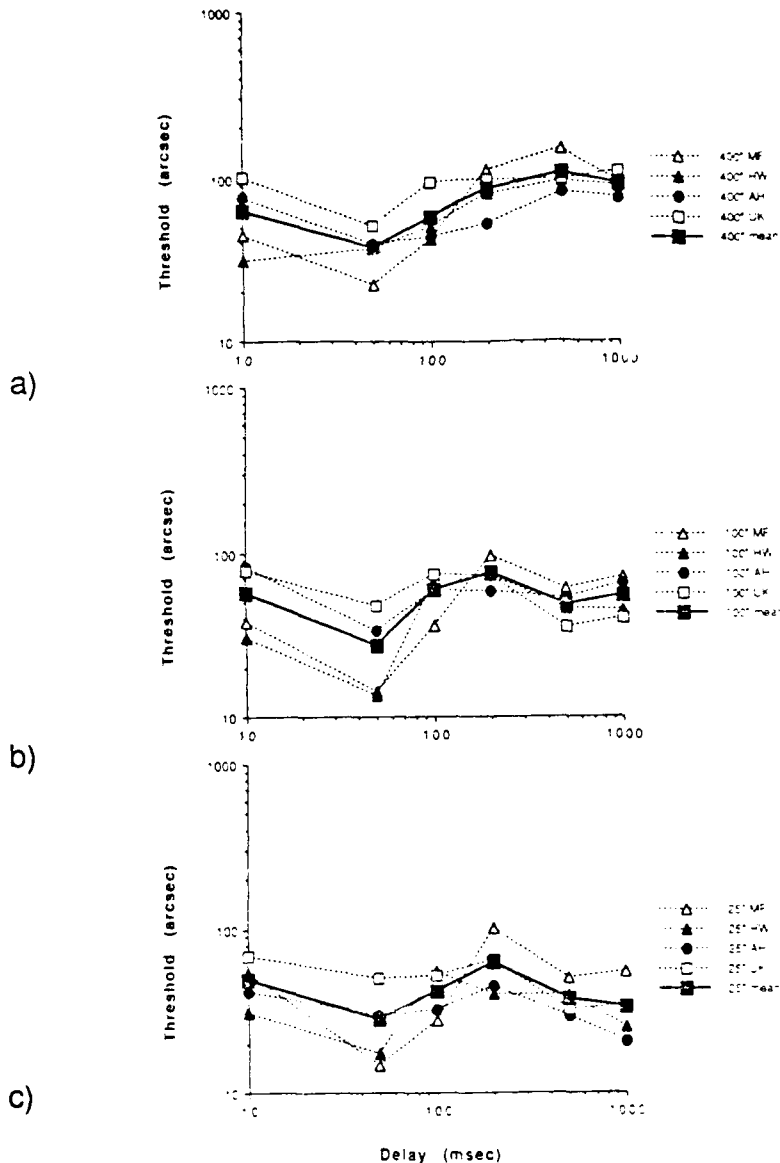
Fig. 5 Monocular vernier thresholds for comparing two vernier targets in the presence of a standing disparity of a) 400", b) 100", c) 25" in the first vernier of each pair. The second vernier followed after the time indicated on the abscissa. Thresholds represent the difference in vernier offset between the first and second verniers.
