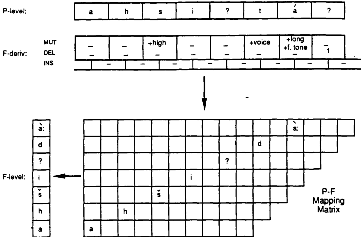
Figure 2: The mapping from P to F level.
