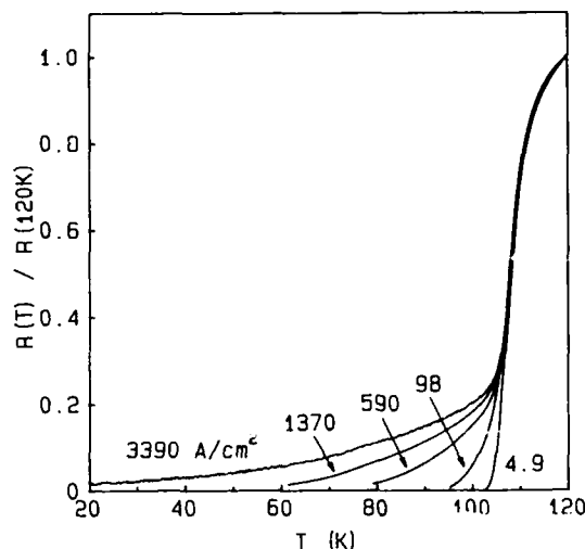
FIG. 3 Normalized resistance of a Bi 1-x Pb x Sr 2 CaCu 2 O 7-x sample using pulse method at various current densities. Sample resistivity at 120 K is 1.1 m \Omega /cm.
