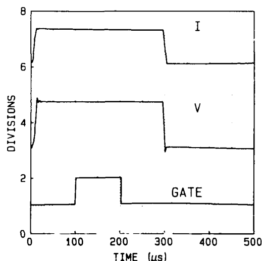
FIG. 2. Digitized photograph of an oscilloscope screen showing current ( I , 0.5\text{ A/division} ), voltage ( V , 0.5\text{ mV/division} ), and gate pulses for a \text{YBa}_2\text{Cu}_3\text{O}_{7-x} sample at a temperature of 84.9\text{ K} .
