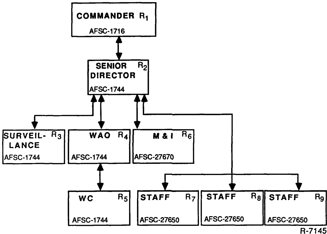
Figure 2-5. Resource Organization
