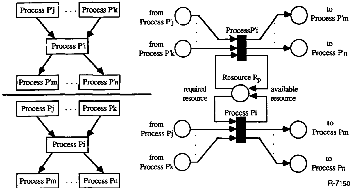
Figure 3-1. Petri Net Representation of R_p Performing P_i and P'_i in any Order.
