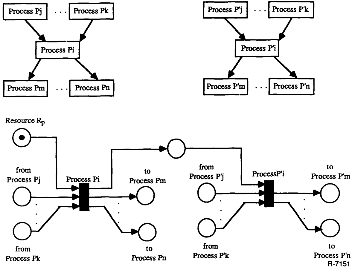
Figure 3-2. Petri Net Representation of R_p Performing P_i First and then P'_i .
