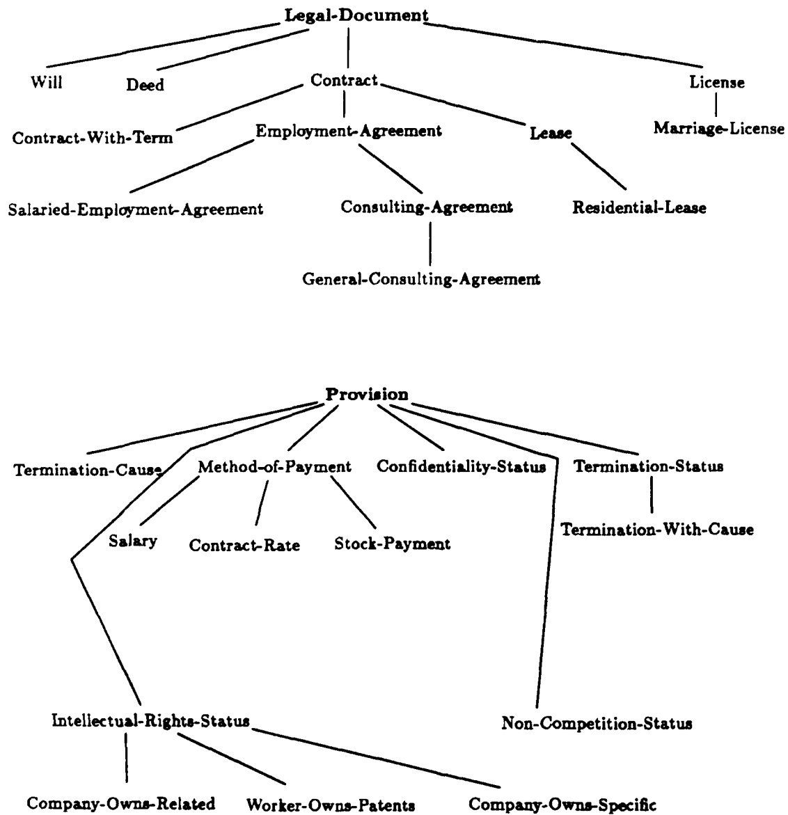
Figure 4-1: Legal Cliché Library
