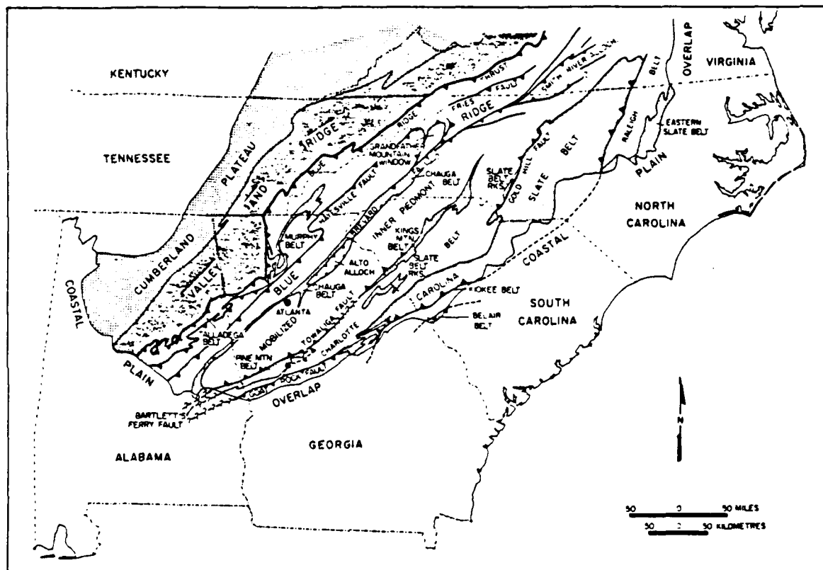
Figure 2. Map of tectonic subdivisions of southern Appalachians (From Hatcher, 1978).
