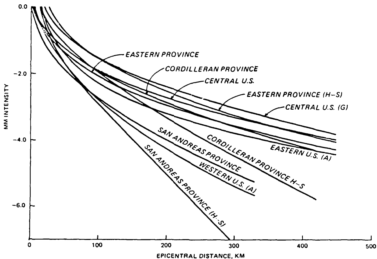
Figure 13. Attenuation of MM Intensity with distance ( A = Anderson, G = Gupta. H-S = Nowell and Schultz). From Chandra, 1979
