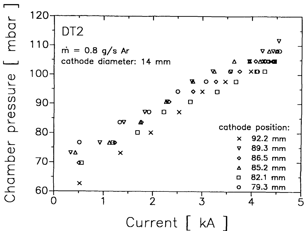
Fig. 2.1.20: Chamber pressure vs. current at various cathode positions
