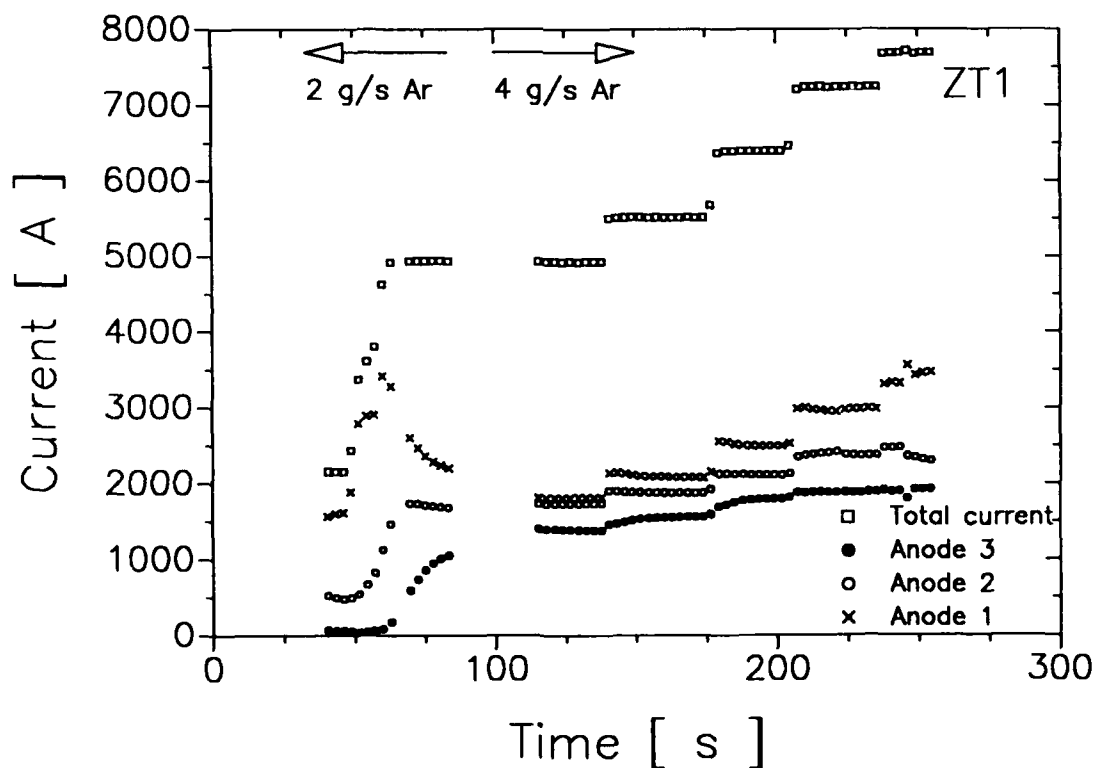
Fig. 2.3.6: Current distribution as a function of time
