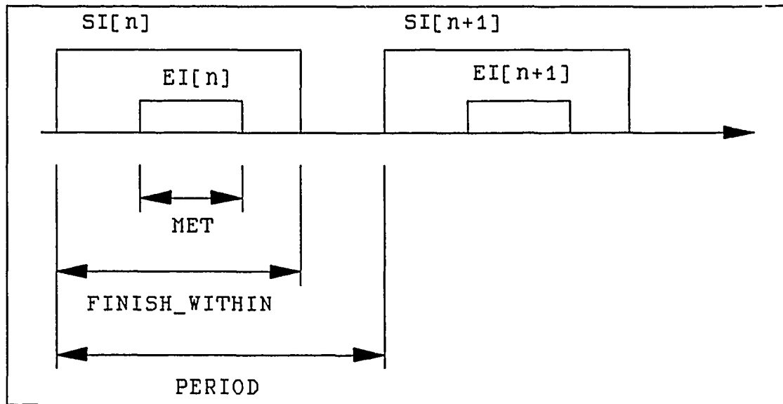
Figure 17 Timing Constraints for a Periodic Operator
