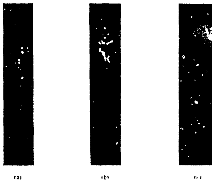
FIGURE 4. EFFECT OF BEARING CLEARANCE ON CAVITATION ( U/D = 0.25 , C_s = 0.4 , U_j = 0.0 RAD/S). C_s = 0.4 , U_j = 0.0 RAD/S. (a) R/C = 89.0, U_b = 104.77 RAD/S, CAVITATION DURATION = 0.13 T. (b) R/C = 201.0, U_b = 104.77 RAD/S, CAVITATION DURATION = 0.23 T. (c) R/C = 201.0, U_b = 146.61 RAD/S, CAVITATION DURATION = 0.33 T.
