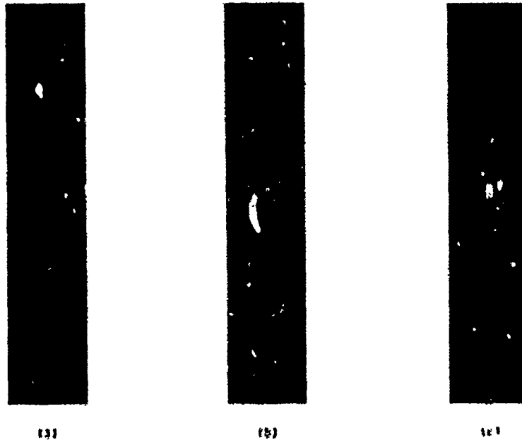
FIGURE 5. - EFFECT OF JOURNAL ROTATION ON CAVITATION ( R/C = 84.0 , L/D = 0.75 , e_z = 0.4 , e_d = 0.55 ).
