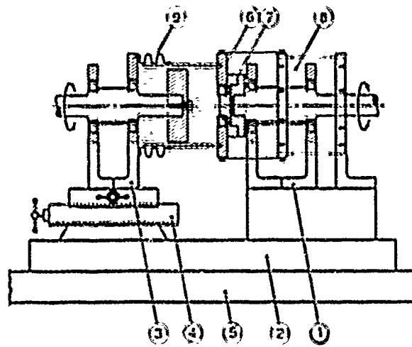
(a) SCHEMATIC.
