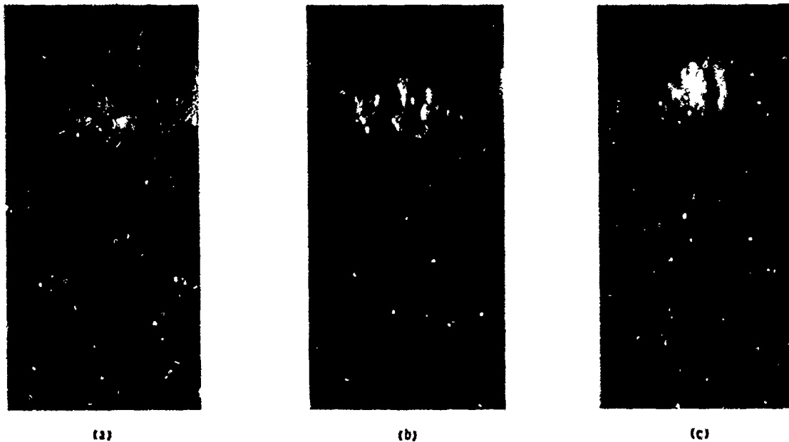
FIGURE 6. - EFFECT OF JOURNAL ROTATION ON CAVITATION ( R/C = 84.0 , L/D = 0.5 , e_z = 0.4 , e_d = 0.55 ).
