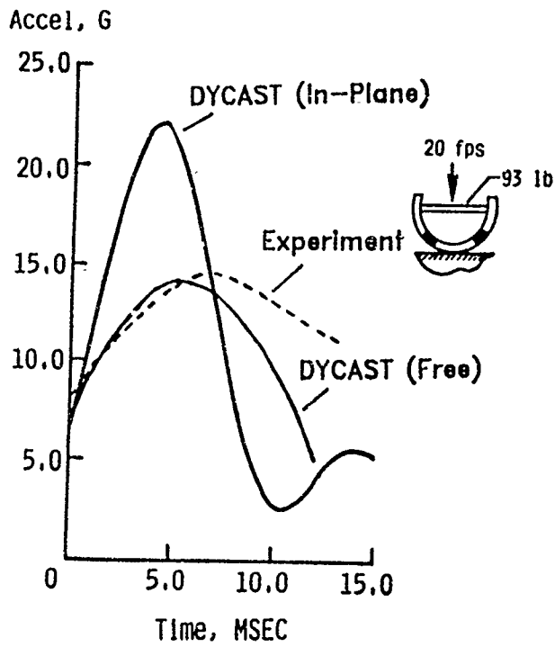
(c) Experimental and analytical accelerations.
