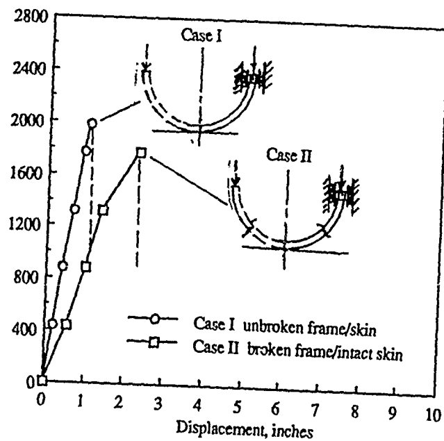
(a) Load-displacement.
