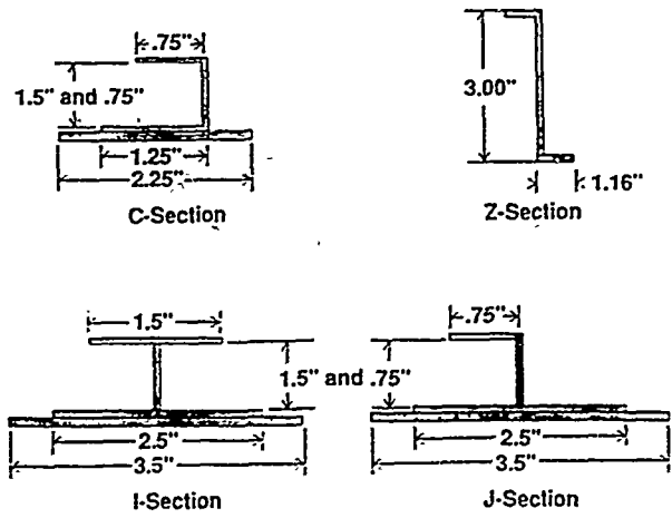
(a) Cross-sectional dimensions.
