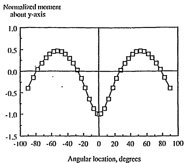
(b) Case I---Normalized moment (Prior to failure).
