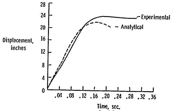
(a) Vertical floor displacement.
