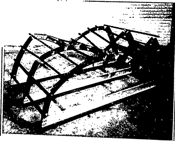
(a) Failed composite skeleton subfloor.
