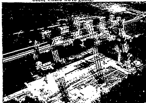
Figure 2. - Impact Dynamics Research Facility (IDRF) at NASA Langley Research Center.
