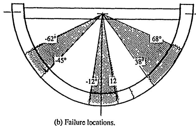
Figure 18. - Comparison of non-dimensional analytical moment distribution predicted by finite element frame model and observed failure locations on metal and composite fuselage components and structures.
