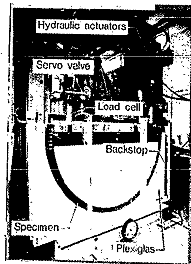
(a) Static test apparatus.
