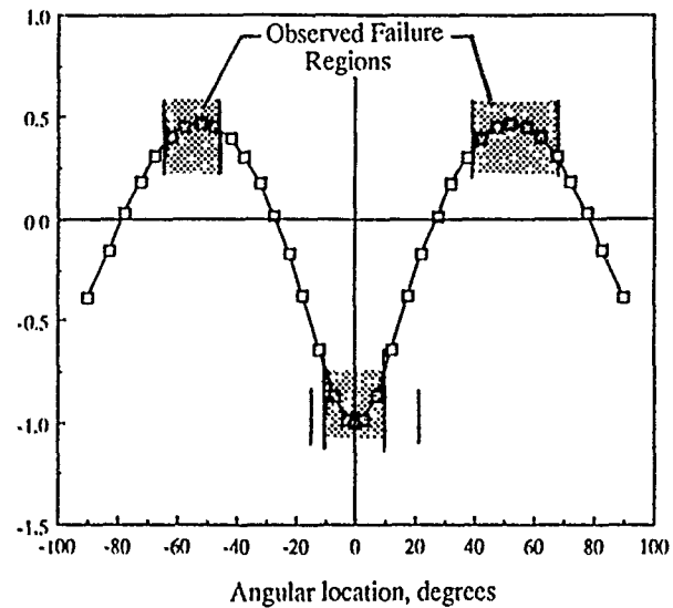
(a) Normalized moment distribution.
