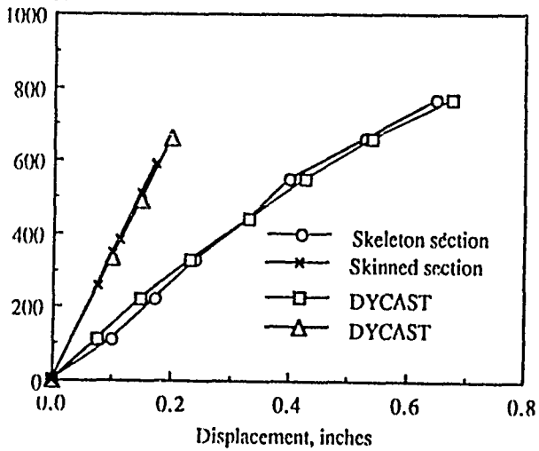
Figure 17. - Comparison of experimental and analytical stiffness of composite skeleton and skinned subfloors.
