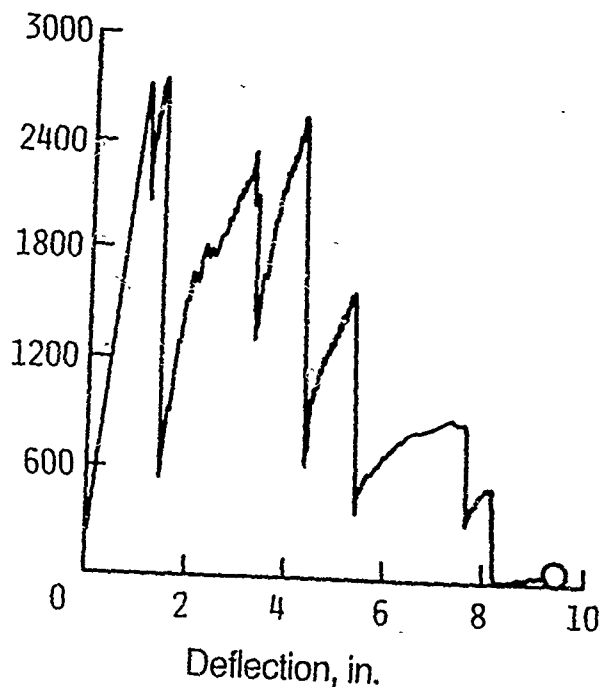
(b) Load-displacement and failure locations.
