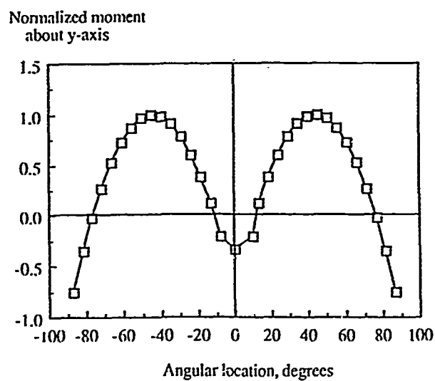
(c) Case II---Normalized moment (Broken frame-intact skin).
