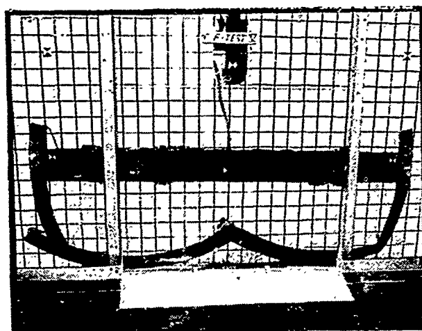
(a) Photographs of failed frames.
