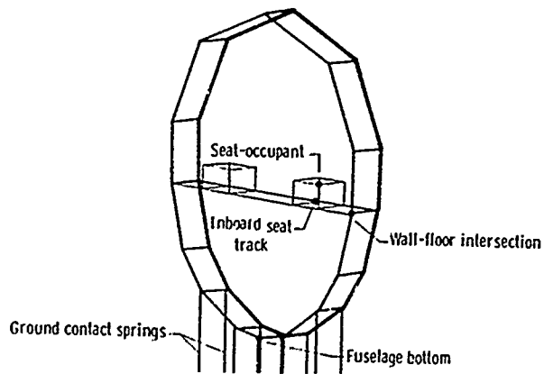
Figure 9. - Finite element two-frame model of metal transport section.
