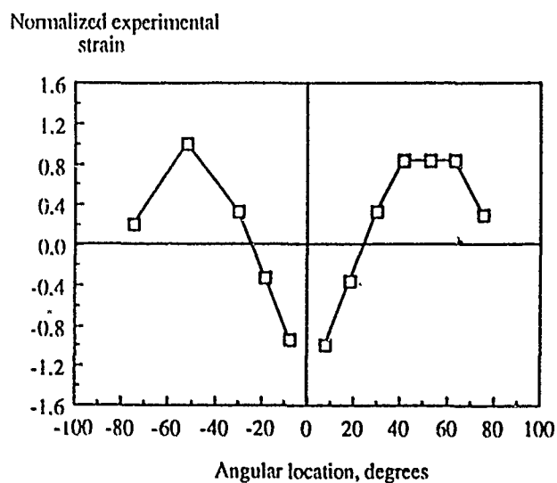
(c) Normalized circumferential strain distribution.
