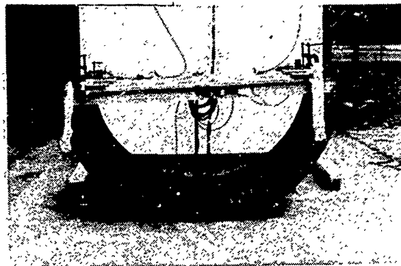
(a) Failed composite skinned subfloor.
