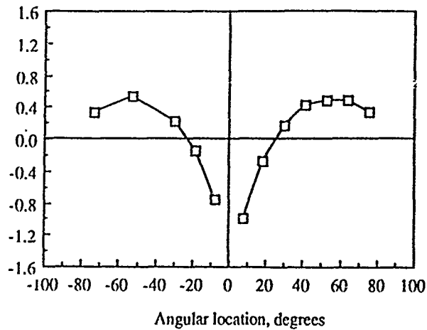
(c) Normalized circumferential strain distribution.
