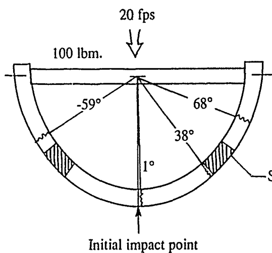
(b) Location of failures in frames.
