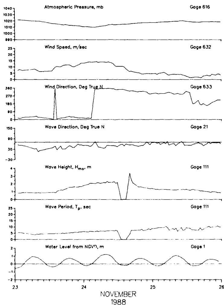
Figure 40. Data for 24 November 1988 storm
