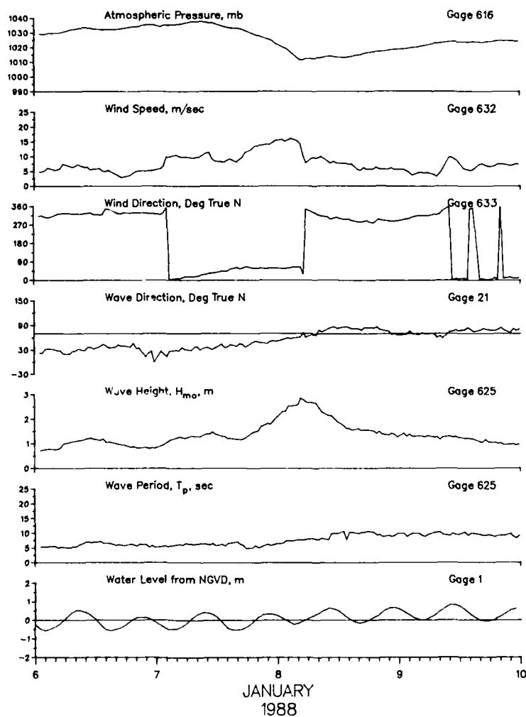
Figure 28. Data for 7-8 January 1988 storm
