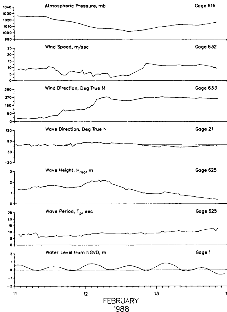
Figure 30. Data for 12 February 1988 storm
