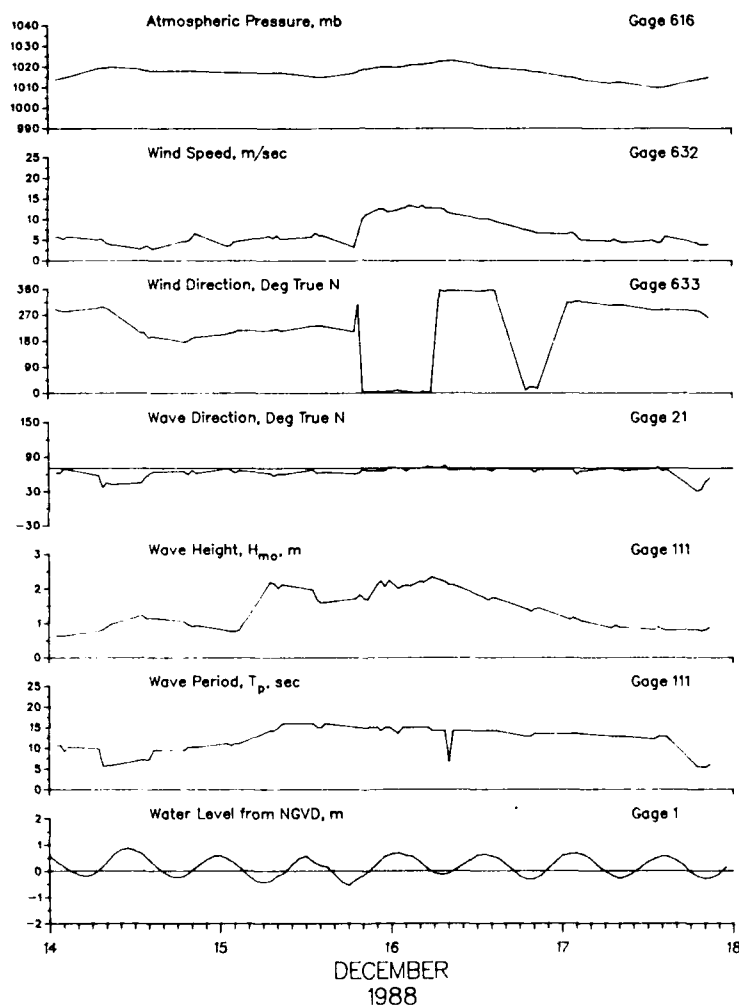
Figure 41. Data for 4 December 1988 storm
