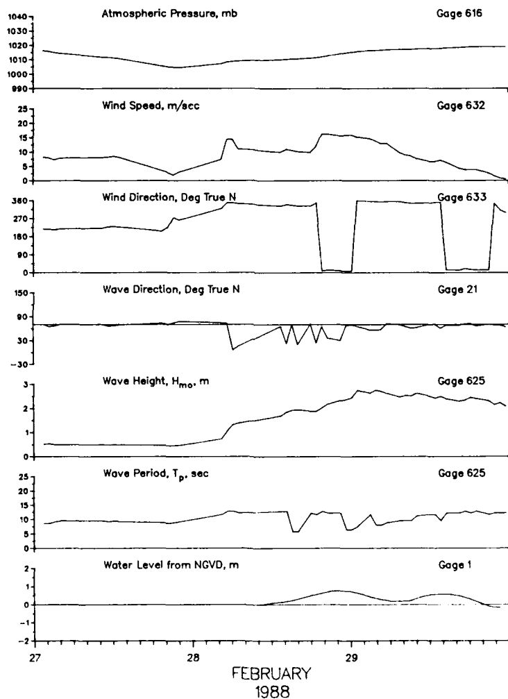
Figure 31. Data for 28 February 1988 storm
