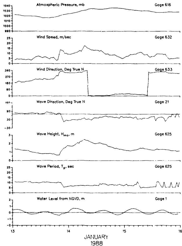
Figure 29. Data for 14 January 1988 storm
