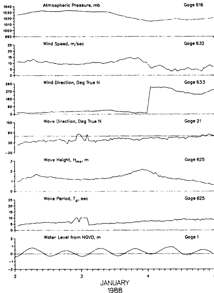
Figure 27. Data for 3 January 1988 storm
