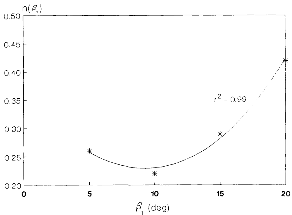
Figure 41. Function n(\beta_1)
