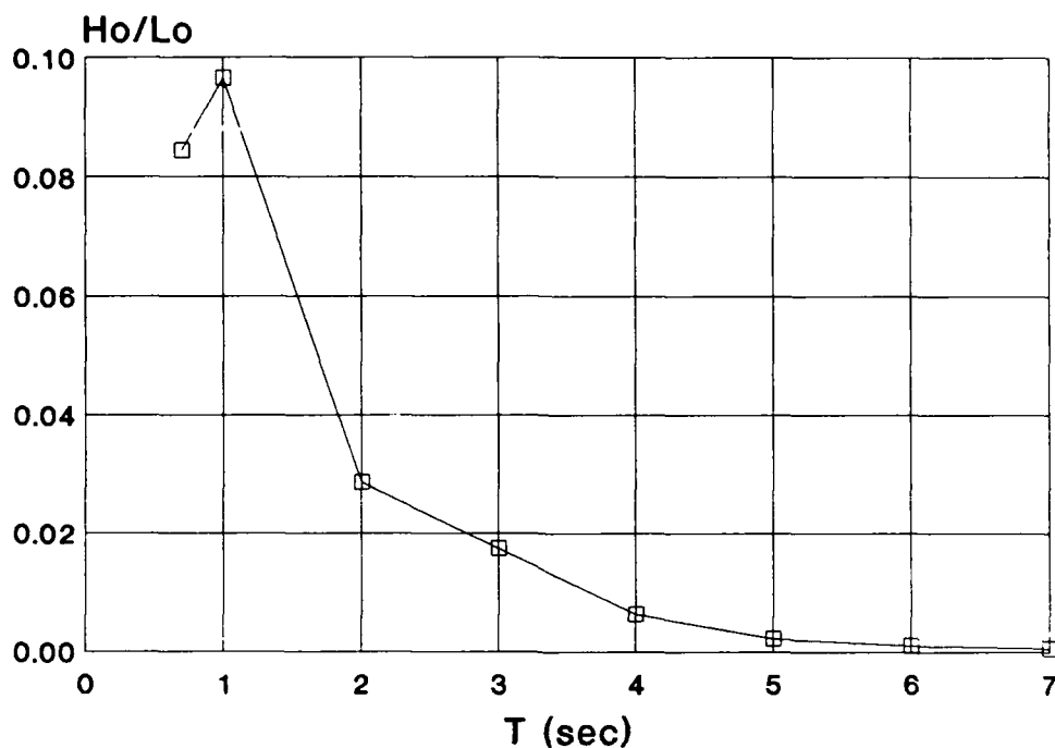
Figure 24. Maximum H_o/L_o as a function of T
