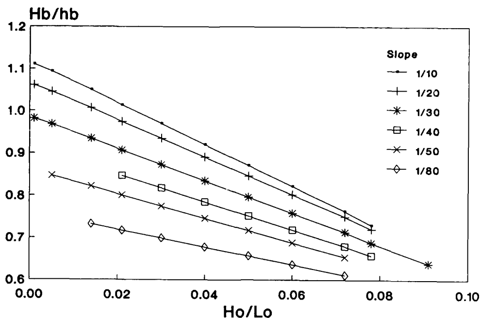
Figure 12. Calculated values of \gamma_b for plane slopes as a function of H_0/L_0
