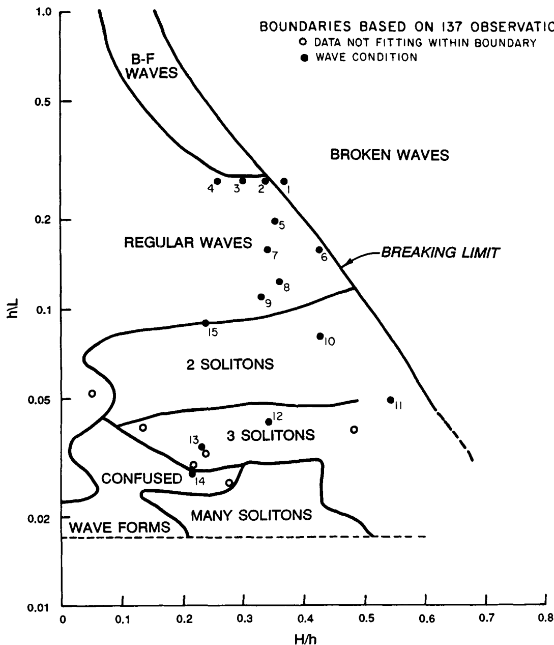
Figure 25. Predicted wave forms produced by a periodic wave generator, after Galvin (1970)
