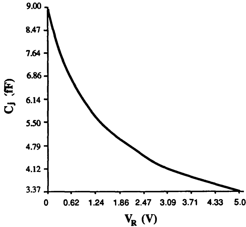
Figure 3-7. Junction capacitance as a function of reverse bias voltage for a 10\text{ }\mu\text{m} \times 10\text{ }\mu\text{m} photodetector.
