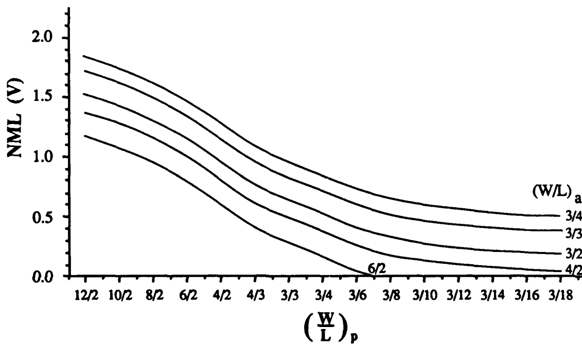
Figure 2-8. CMOS Static RAM Cell Low Noise Margin. Data are for selected PMOS transistor sizes with access transistor aspect ratio as a parameter and (\frac{W}{L})_n = 3/2 .
