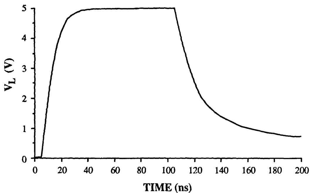
Figure 4-9. Transient Response of the Detector and Saturated NMOS Load.
