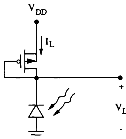
Figure 4-15. Photodetector with a Saturated PMOS Pull-Up Load.
