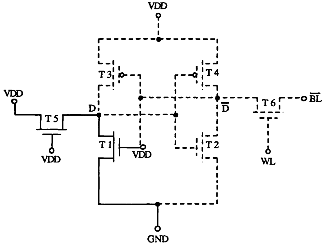
Figure 2-5. CMOS SRAM Cell Read Access Inverter.
