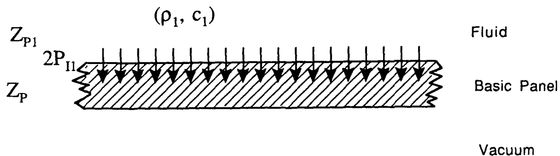
Fig. 4. A plane dynamic system consisting of a basic panel facing a fluid and backed by vacuum. The surface impedances of the fluid and the basic panel and the blocked incident pressure are indicated [cf. Fig. 1.].
