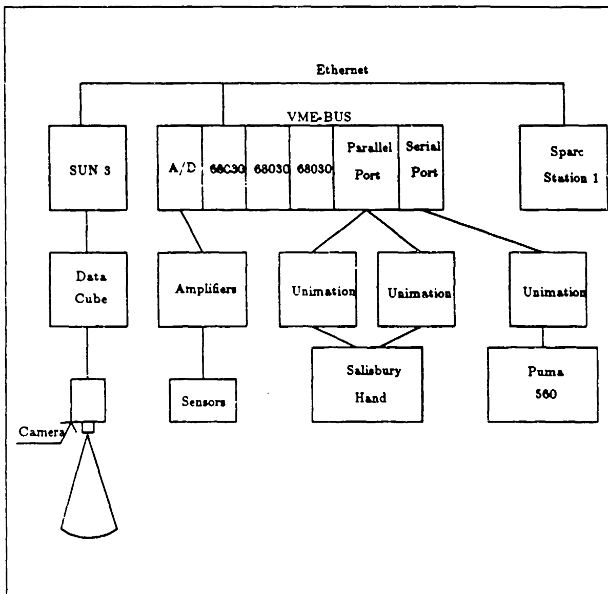
Figure 7.1: 3-D Experimental Set-Up
