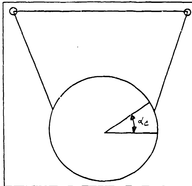
Figure 2.4: Form Closure Grasps Relying on Friction
