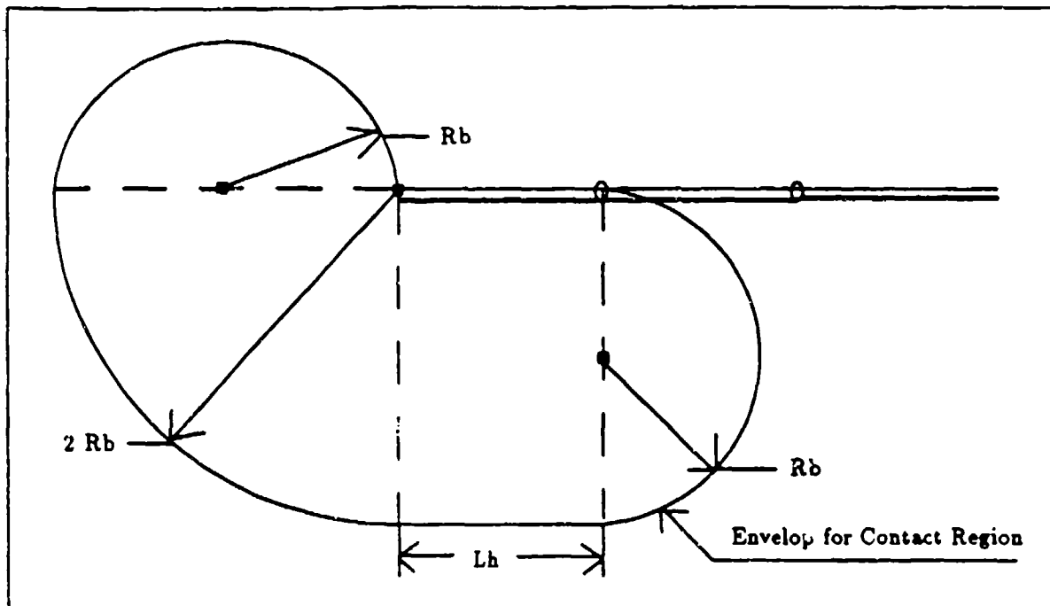
Figure 3.6: First Contact Region
