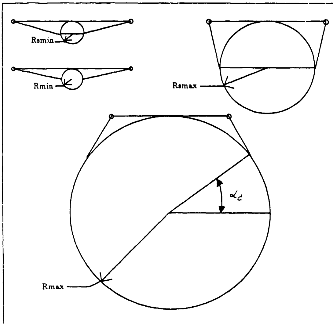
Figure 2.5: Illustration for Minimum and Maximum Graspable Cylinder Radius (for Structural Form Closure, R_s , and Frictional Force Closure, R_f )
