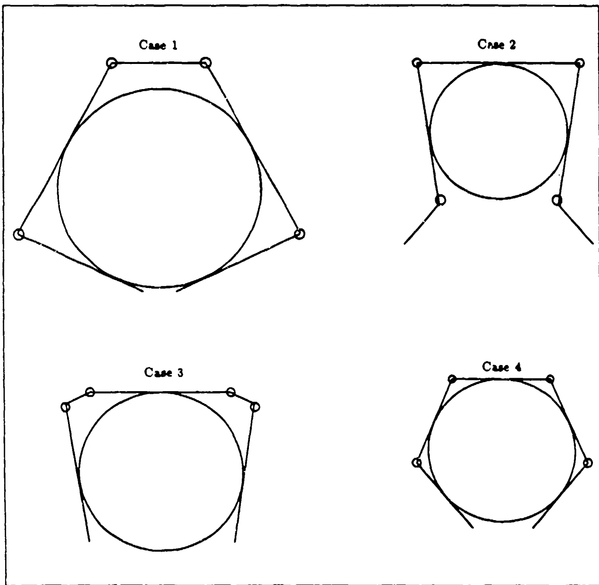
Figure 5.2: Four Possible Structural Form Closure Grasps
