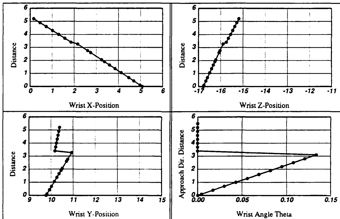
Figure 4.5: Plots of wrist parameters against distance remaining in the approach. \mathbf{k} is [-.867 \ -.004 \ .498]^T , z is up from the table, y is away from the block, and the approach direction is roughly in the x -direction.
