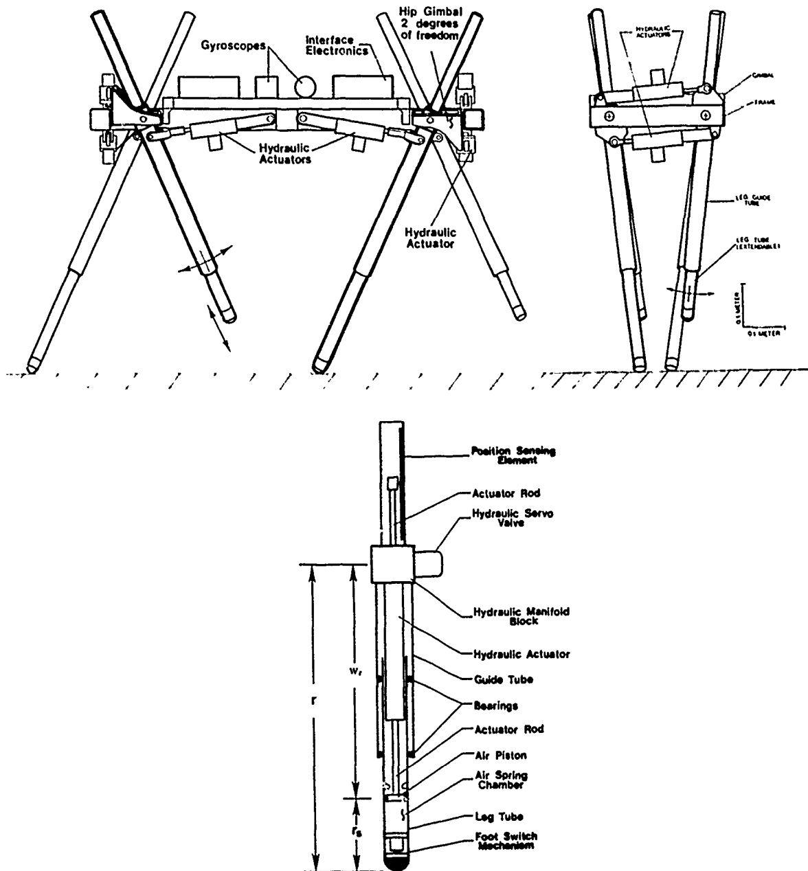
Figure 6-4: Diagram of quadruped running machine used for experiments. The body is an aluminum frame, on which are mounted legs, hip actuators, gyroscopes, and computer interface electronics. Each hip has two low friction hydraulic actuators that position the leg fore and aft, and sideways. Sensors measure the position, velocity, and force of the hydraulic hip actuators, hydraulic leg length, overall leg length, leg spring length, contact between the feet and the floor, and the pitch, roll, and yaw orientations of the body. An umbilical cable connects the machine to hydraulic, pneumatic, and electrical power supplies, and to the control computer (VAX/785), all of which are located nearby in the laboratory. The arrangement of spring in series with position source in each leg was motivated by simple muscle models. Physical parameters of the quadruped machine are given in table 6-1.
