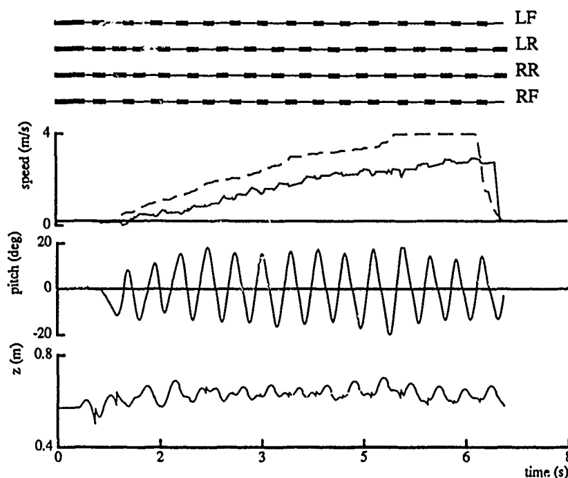
Figure 6-13: Bounding with independent state machines for front and rear virtual legs. The machine started bounding in place, accelerated up to 3 m/s, and stopped abruptly just before reaching the end of the laboratory. Once again, there is a substantial discrepancy between the desired forward running speed (shown dashed) and the measured running speed. As the machine increased speed, the phase relationship between front and rear ground impacts shifted away from 180^\circ . (Data file C637.196.4.)
