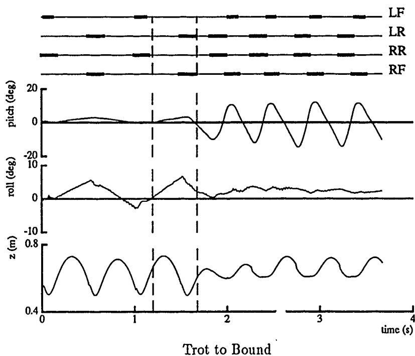
Figure 6-14: Gait transition: Top) Data recorded during a transition from trotting to pacing. The transition occurred during a flight phase, as indicated by the vertical dashed line. There was little disruption of the running motion. Forward running speed was essentially zero. Bottom) The transition from trotting to bounding took several steps to stabilize. The vertical dashed lines bracket the transition step, which induced pitching of the body. ((Data file Q87.335.3 and Q88.2.3.)
