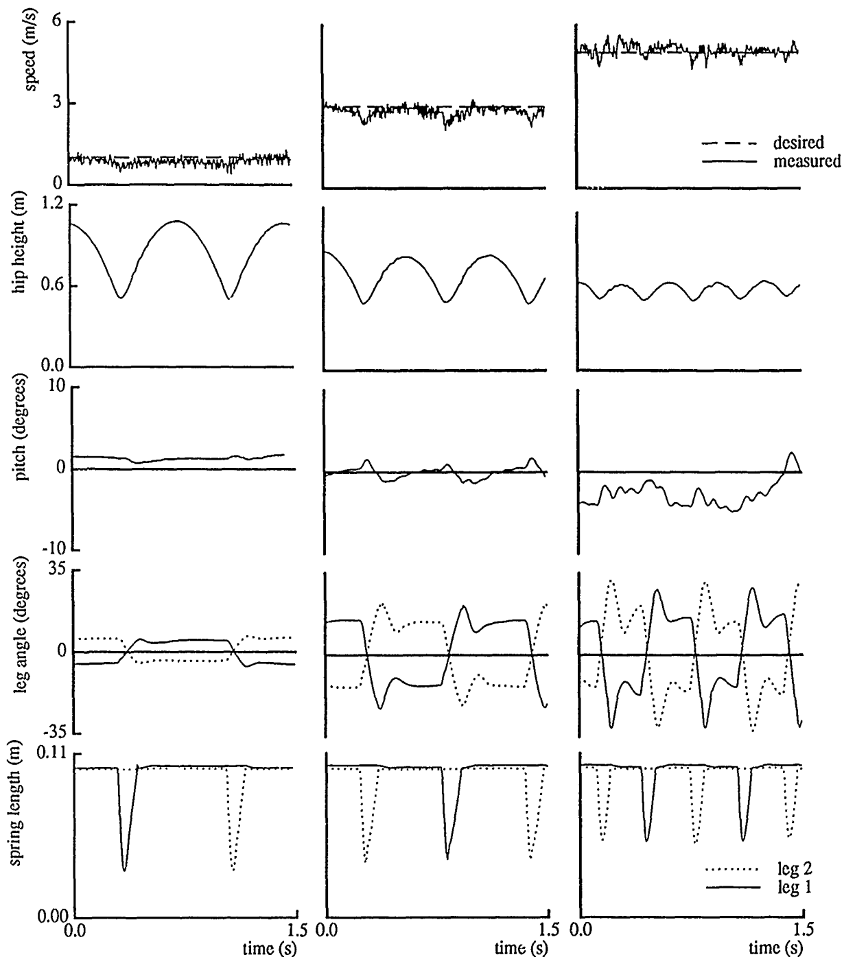
Figure 4-7: The planar biped ran forward at 1, 3, and 5 m/s. The top three graphs show the forward speed, hip height, and pitch angle of the body. The fourth graph shows the equal and opposite motions of the two legs as they sweep back and forth. The bottom graph shows how the two leg springs compressed as the biped bounced alternately on the two feet. As running speed increased, the frequency of stepping and leg angle excursion increased, and the compression of the legs during the bounce decreased. (Data files B88.241.4, B88.241.3, B88.241.1)
