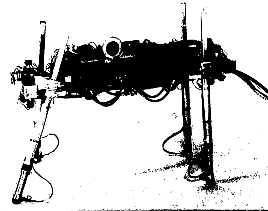
Figure 6-1: Photograph of quadruped running machine used for experiments.
