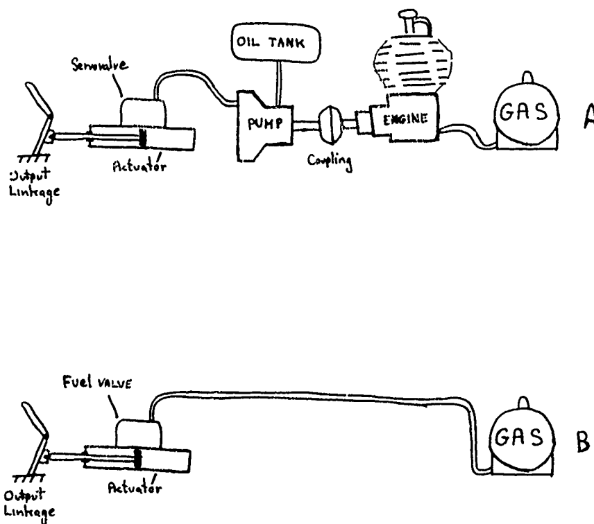
Figure 9-1: A) A conventional power system employing an internal combustion engine, a hydraulic pump, and hydraulic servoactuators. B) An internal combustion actuator . The engine, coupling linkages, and hydraulic pump are eliminated, since the fuel is combusted directly in the linear actuator.
