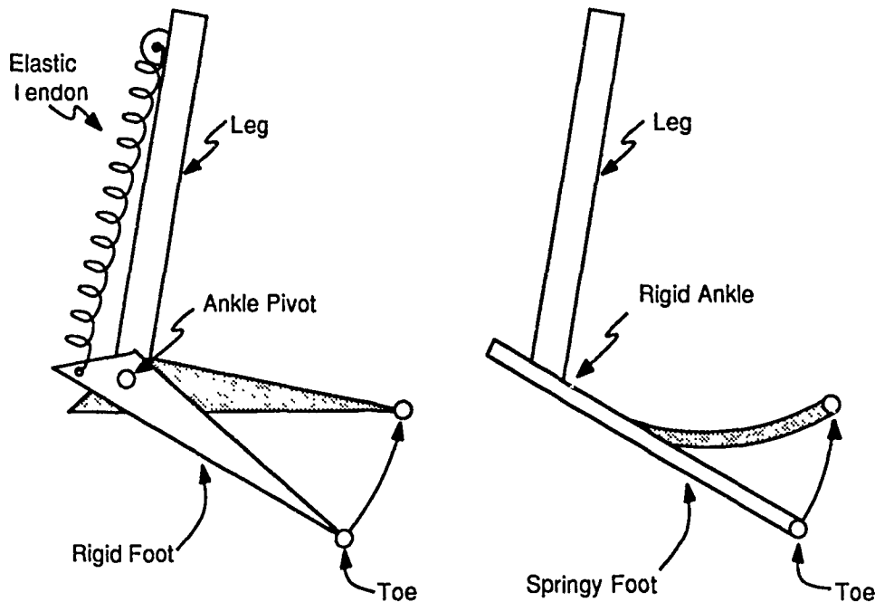
Figure 8-6: Articulated legs. Left) An anthropomorphic design uses a hinged, inflexible foot with a springy tendon. Right) Alternate design employs bending of an elastic foot to provide springiness.
