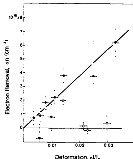
FIG. 1. Electron removal \Delta n vs the degree of deformation \Delta l/l_0 . Full circles and full triangles correspond to n -type samples deformed along (111) and (110) directions, respectively. Open circles correspond to p -type samples deformed in the (111) direction. Open triangle denotes the magnitude of electron removal from EL2 in the (100) direction.
