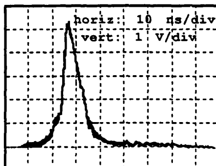
Figure 13. Single mode temporal profile of HyperDYE-300.
