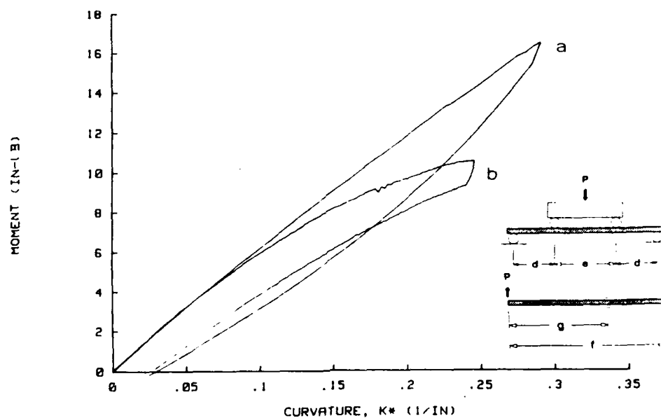
Figure 3.20 Moment-curvature relationship for the \pm 45^\circ angle-ply layup from a) cantilever-type specimen and b) four-point bend specimen. d=3 , e=2 , f=3.980 , g=1.980 .
