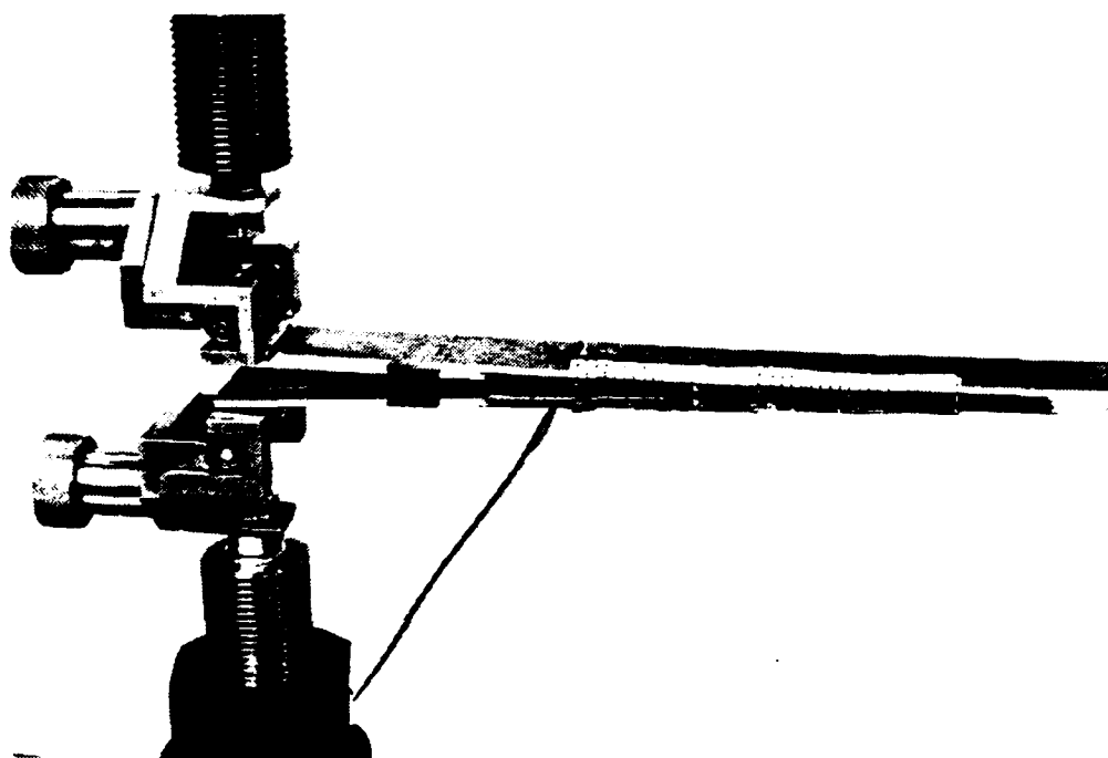
Figure 3.3 DCB specimen with crack propagation gages
