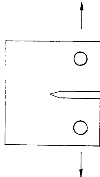
(c) Illustration of CT specimen
