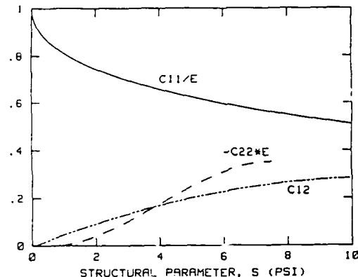
Fig. 2 Coefficients in equation (26) for E = 400 psi (2.76 MPa).
