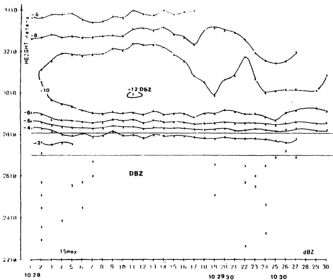
Fig. 9 Time-height display of radar reflectivity contours in the melting zone. Time starts at 10:28:00 and ends at 10:30:30, approximately. The solid line is a melting layer reference also shown in Fig. 10 for comparison between velocity and radar reflectivity data.
