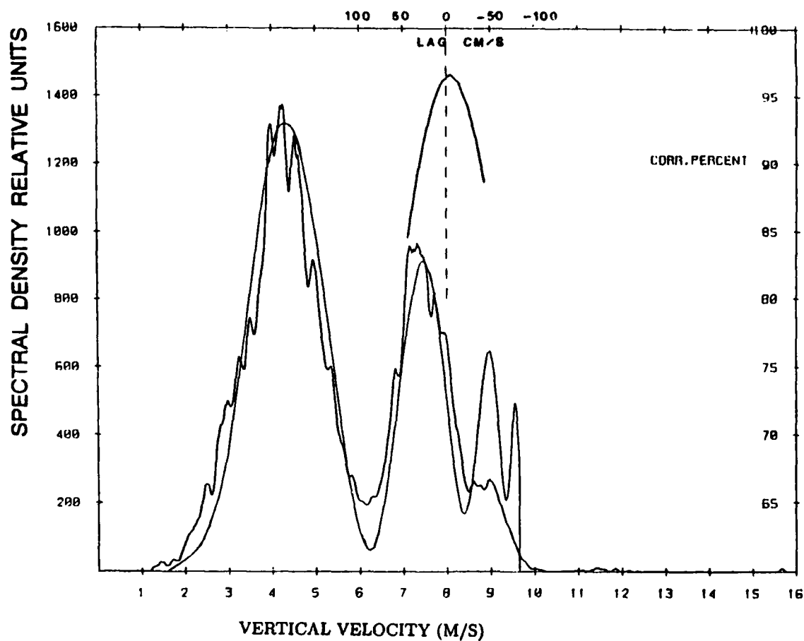
Fig.17 Doppler spectrum observed at vertical incidence together with a predicted spectrum (smooth function) based on the Mie backscattering function and a M-P dropsize distribution with \Lambda adjusted for the best fit of the two maxima. The function at the top of the figure is the cross correlation between the two spectra as a function of the velocity lag indicated by the top scale.
