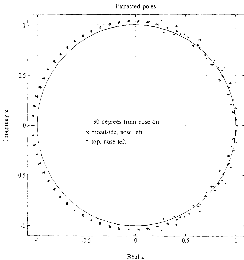
Figure 40. Kumaresan-Tufts Poles, Target 2
