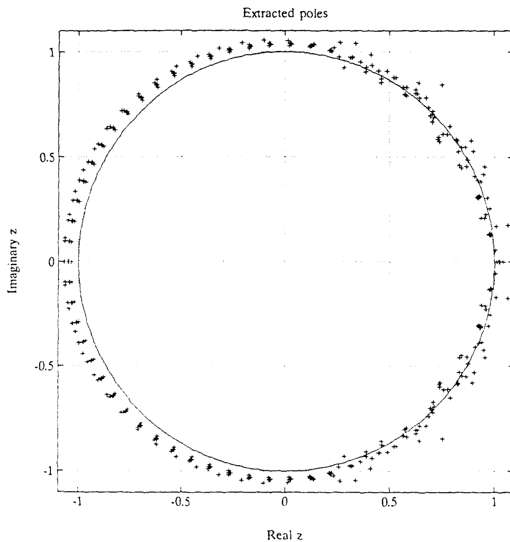
Figure 42. Kumaresan-Tufts Poles, Target 2
