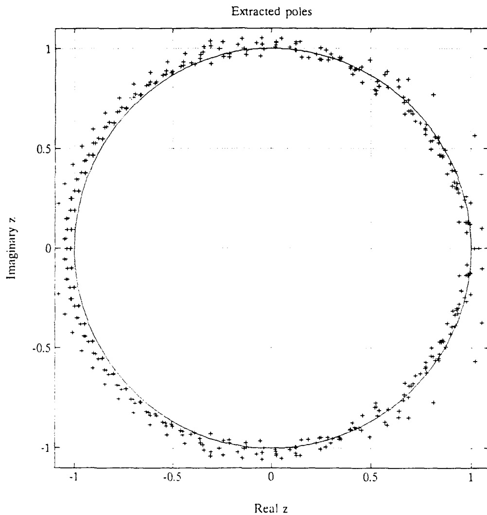
Figure 39. Kumaresan-Tufts Poles, Target 1
