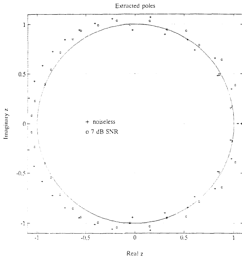
Figure 59. Integral Equation Thin Wire Comparison, Noiseless vs. 7.0 dB SNR, 90 Degree Aspect
