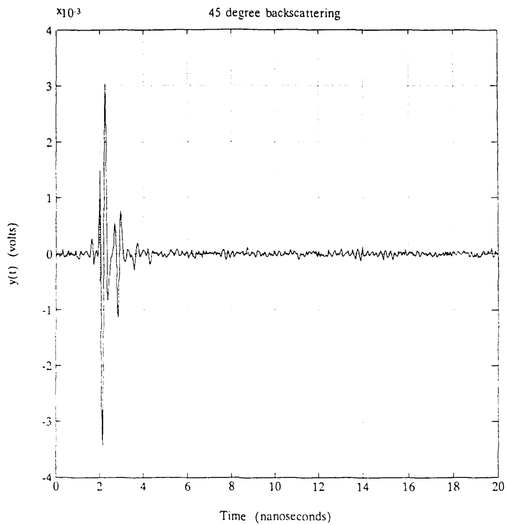
Figure 28. Measured Thin Wire Scattering, 45 Degree Aspect
