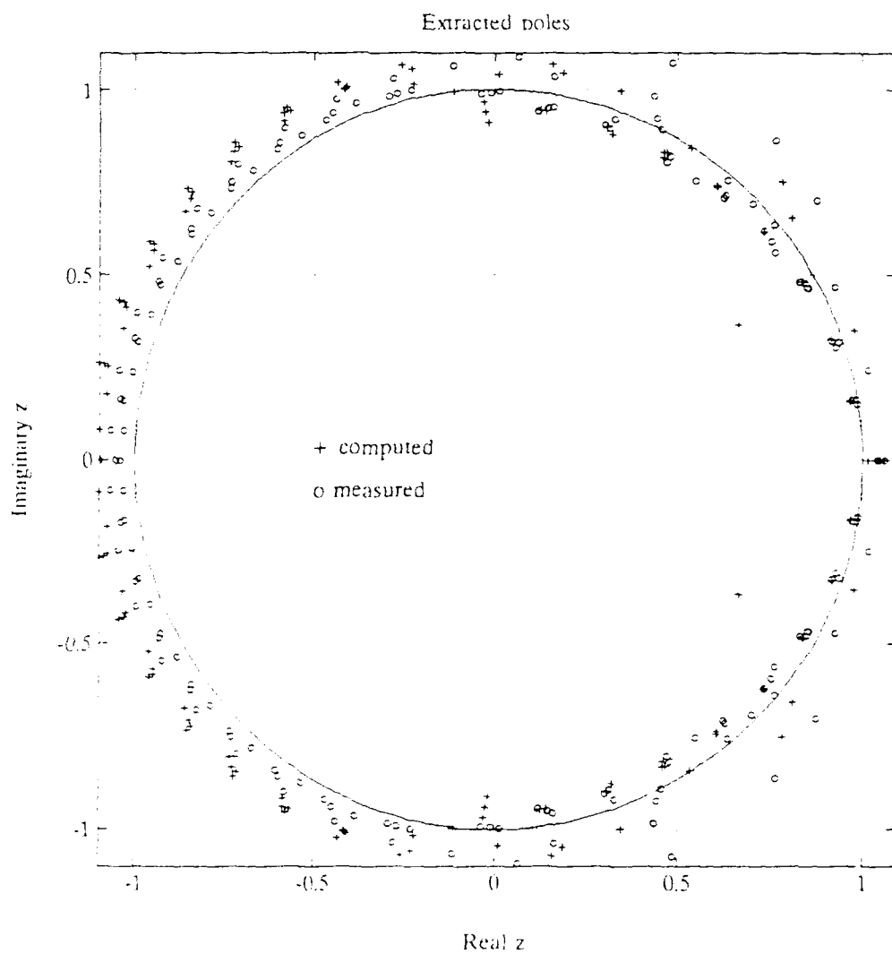
Figure 61. Thin Wire Comparison, Measured vs. Integral Equation
