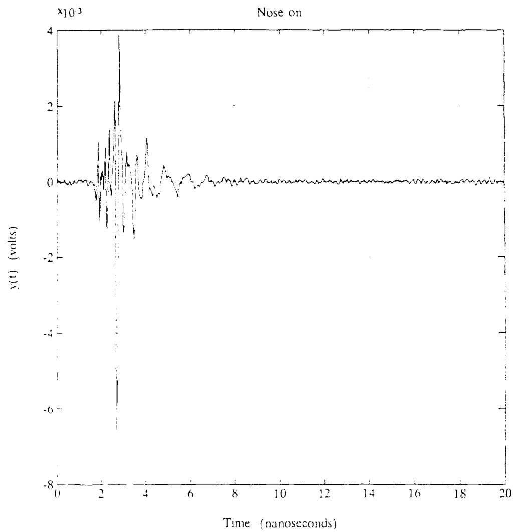
Figure 34. Target 1 Scattering, Nose on
