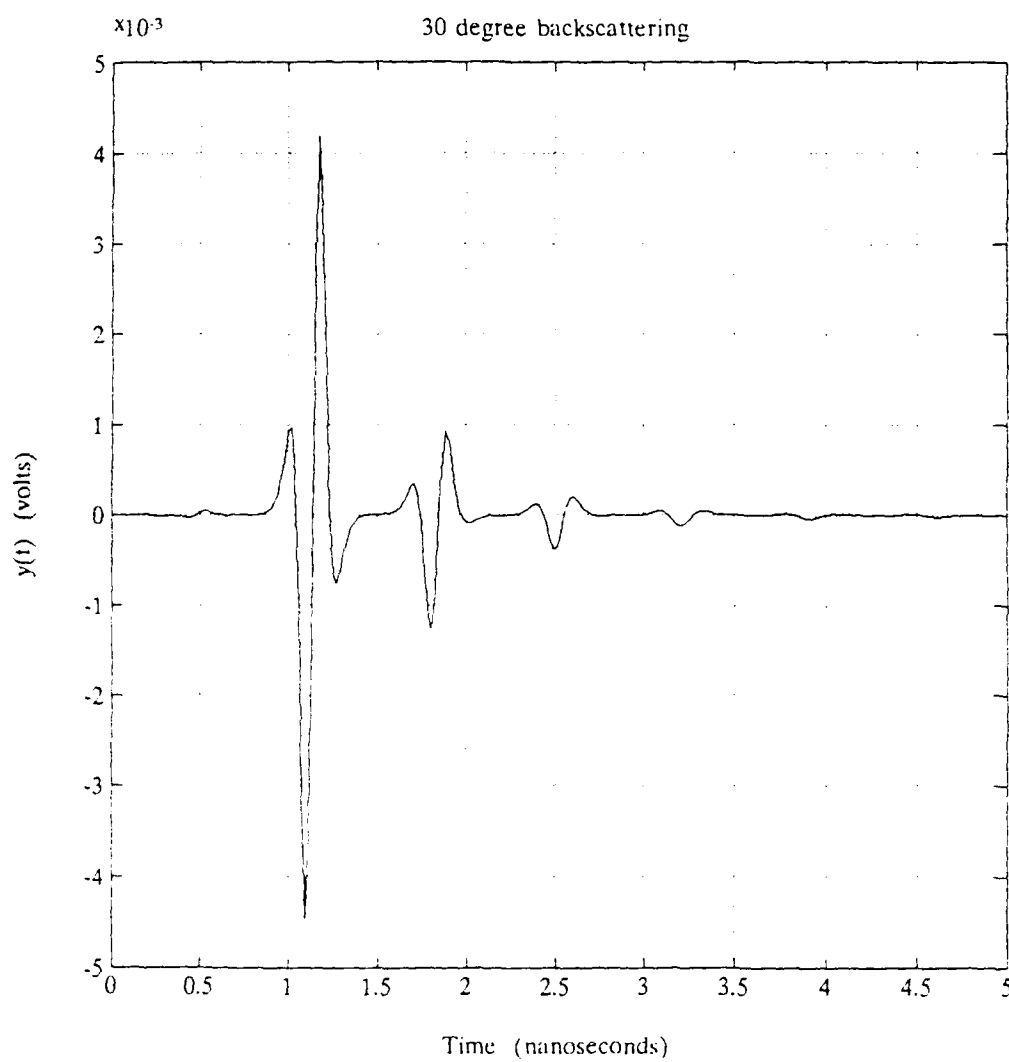
Figure 10. Integral Equation Thin Wire Scattering, 30 Degree Aspect
