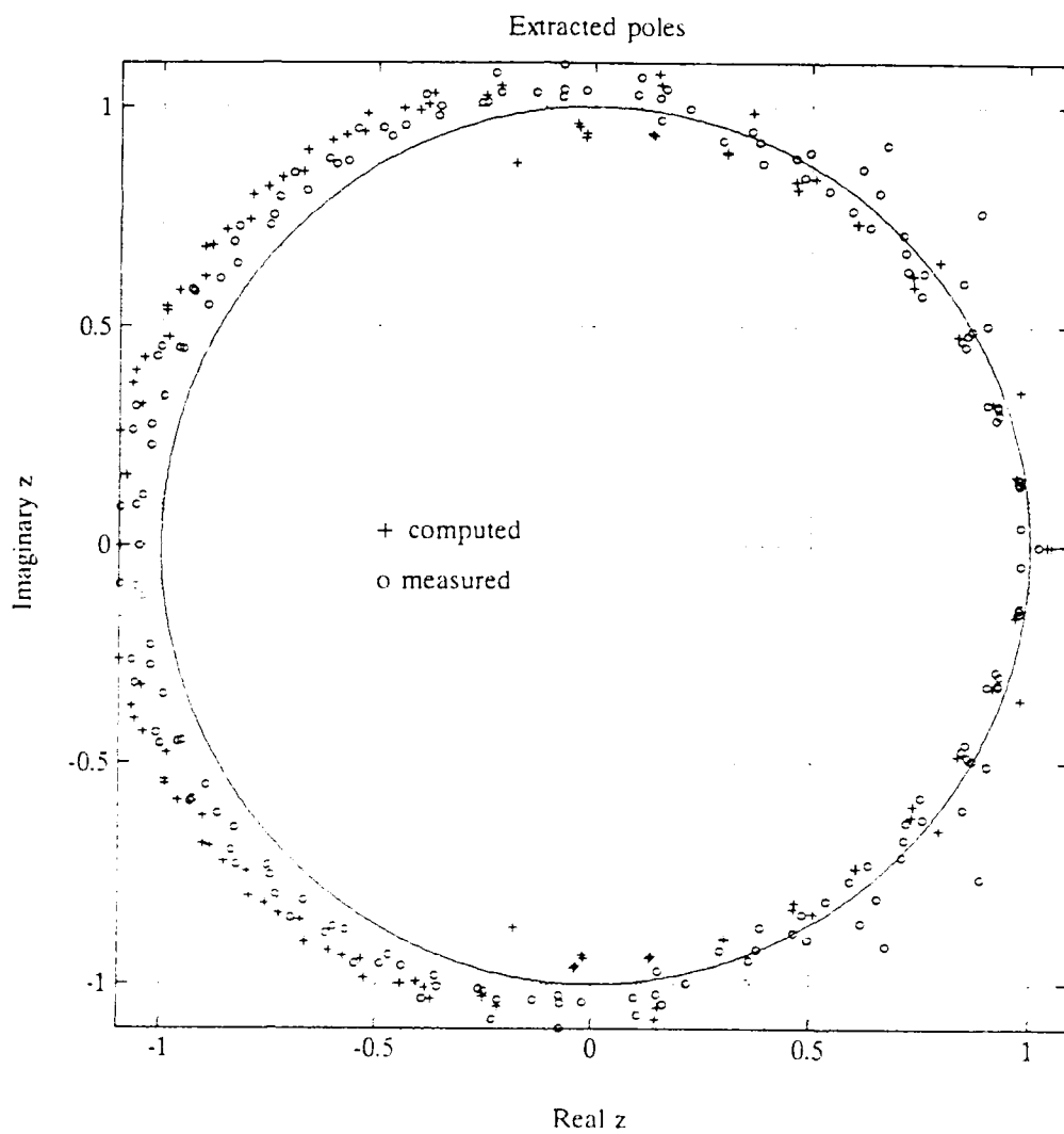
Figure 32. Thin Wire Comparison, Measured vs. Integral Equation
