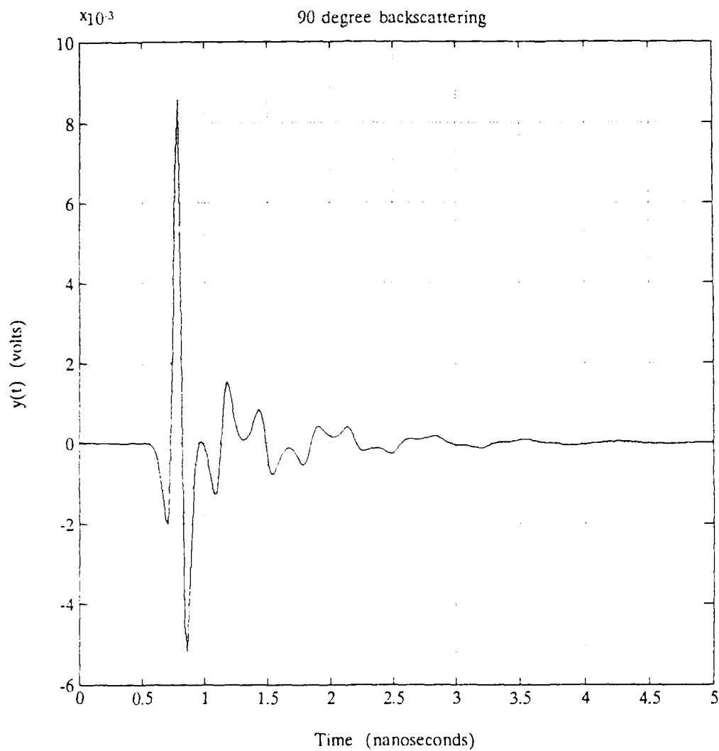
Figure 13. Integral Equation Thin Wire Scattering, 90 Degree Aspect
