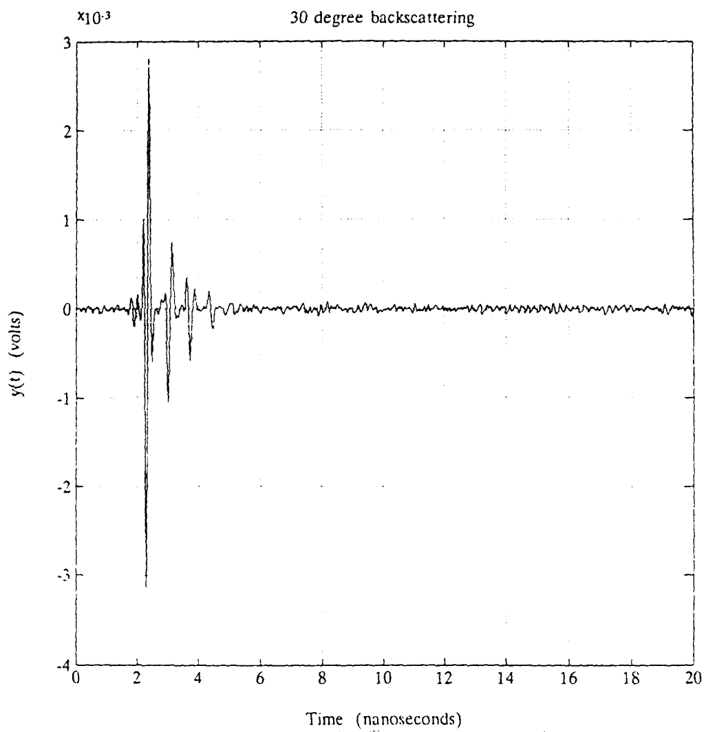
Figure 27. Measured Thin Wire Scattering, 30 Degree Aspect
