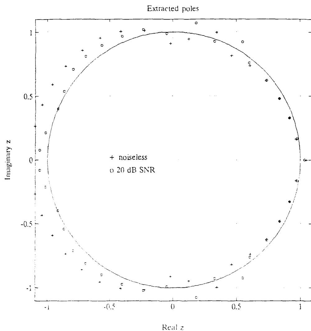
Figure 52. Integral Equation Thin Wire Comparison, Noiseless vs. 20.0 dB SNR, 45 Degree Aspect
