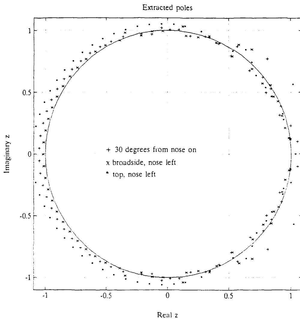
Figure 37. Kumaresan-Tufts Poles, Target 1
