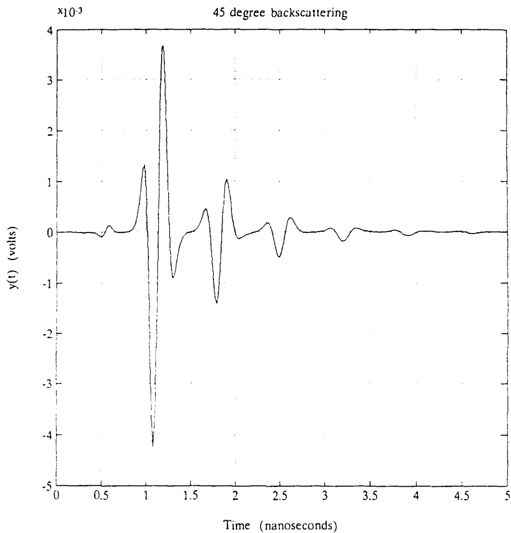
Figure 11. Integral Equation Thin Wire Scattering, 45 Degree Aspect
