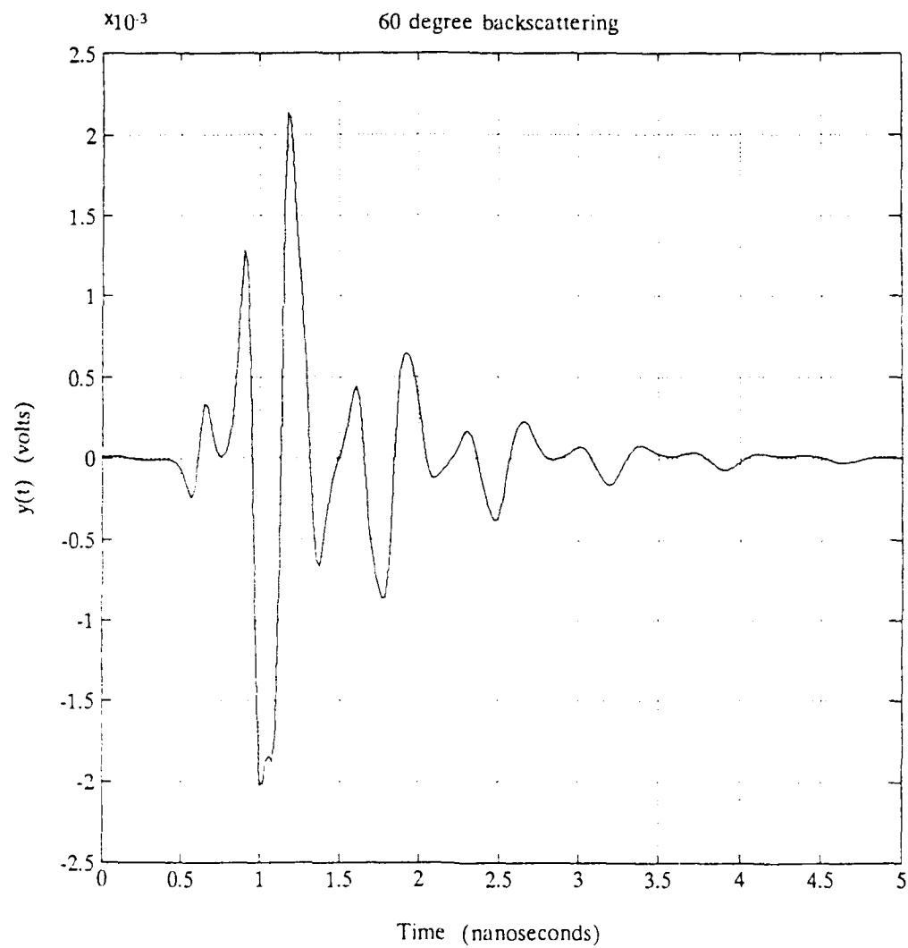
Figure 12. Integral Equation Thin Wire Scattering, 60 Degree Aspect
