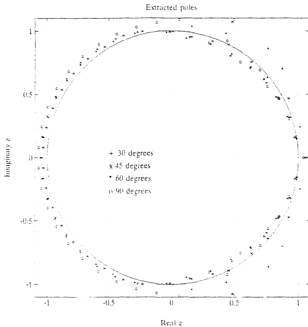
Figure 60. Cadzow-Solomon Poles, Measured Thin Wire
