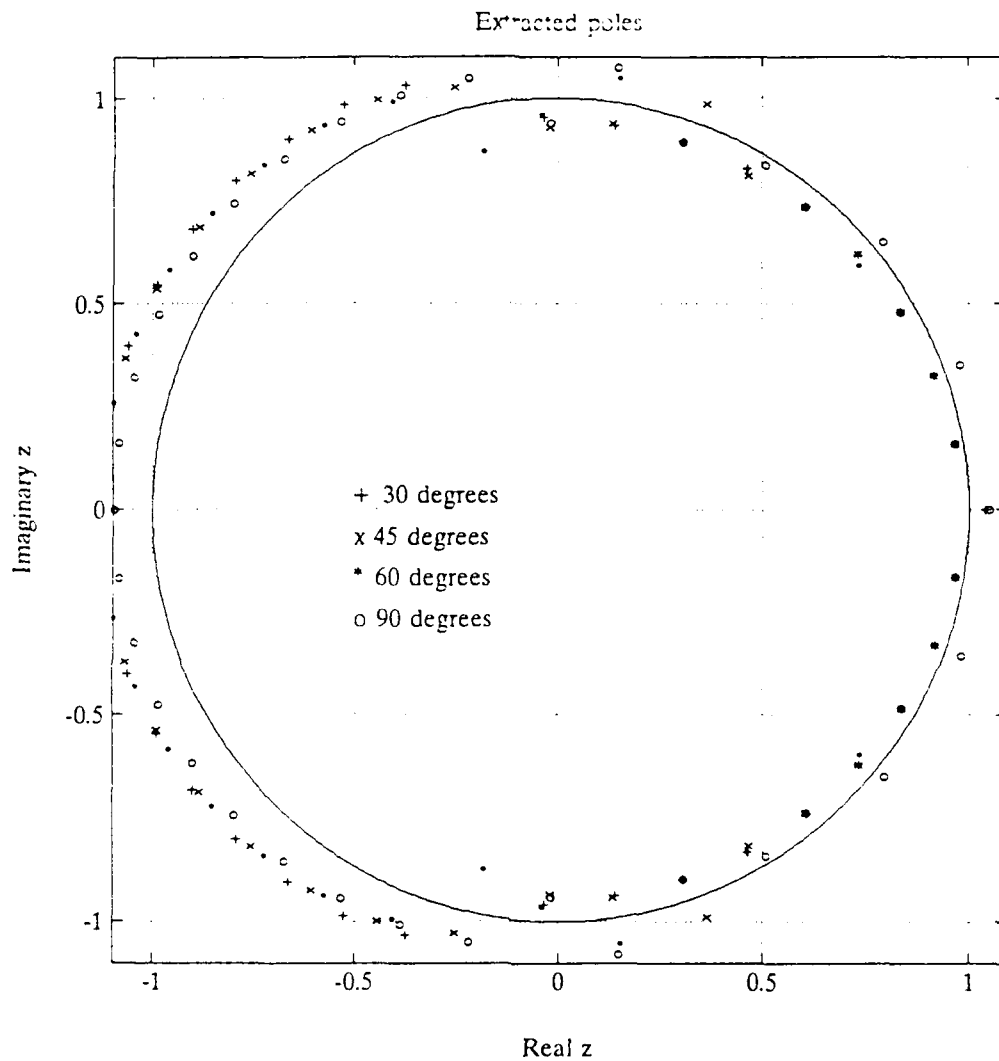
Figure 14. Kumaresan-Tufts Poles, Noiseless Thin Wire Data
