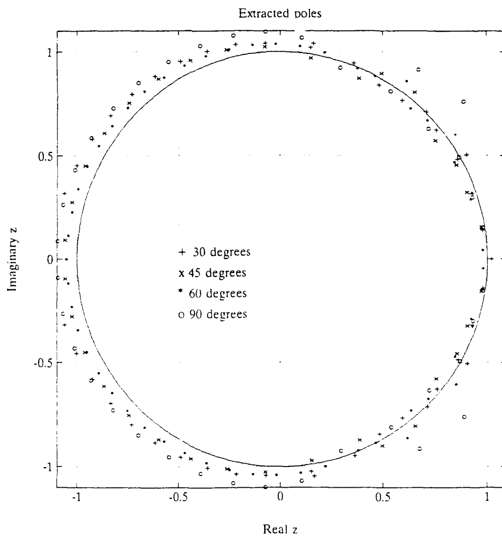
Figure 31. Kumaresan-Tufts Poles, Measured Thin Wire
