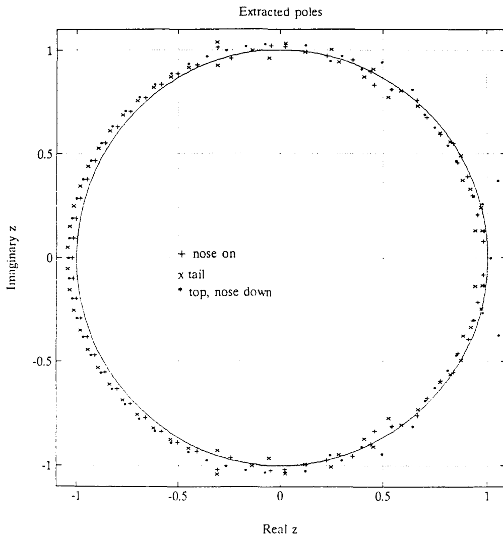
Figure 38. Kumaresan-Tufts Poles, Target 1
