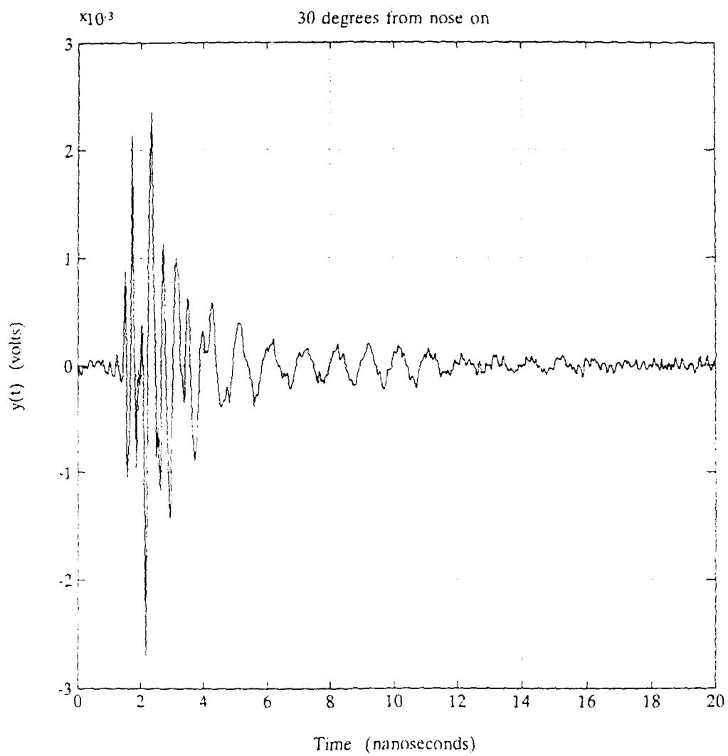
Figure 35. Target 2 Scattering, 30 Degrees from Nose on
