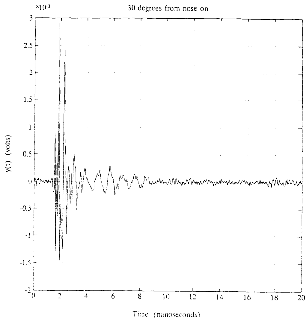
Figure 33. Target 1 Scattering, 30 Degrees from Nose on
