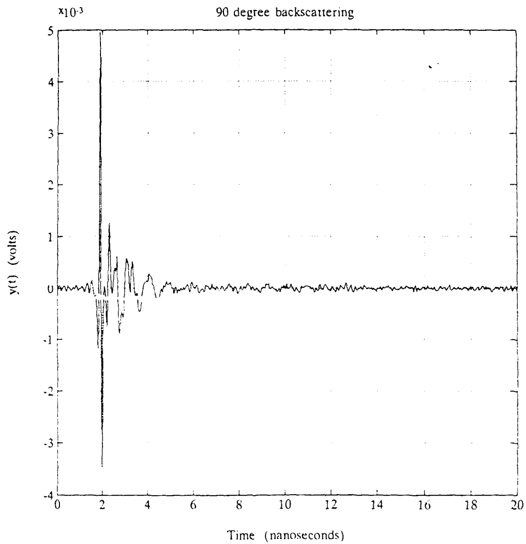
Figure 30. Measured Thin Wire Scattering, 90 Degree Aspect
