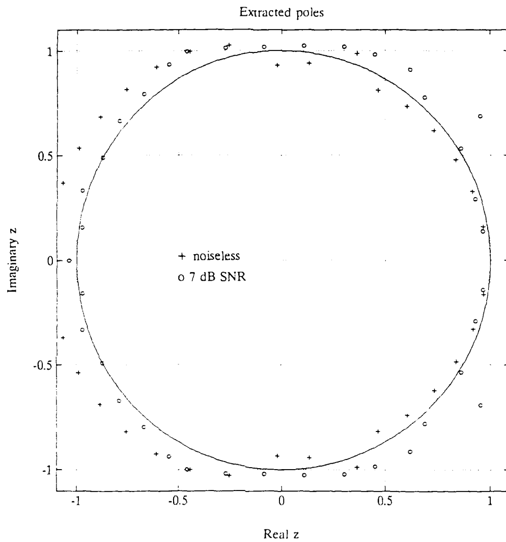
Figure 24. Integral Equation Thin Wire Comparison, Noiseless vs. 7.0 dB SNR, 45 Degree Aspect
