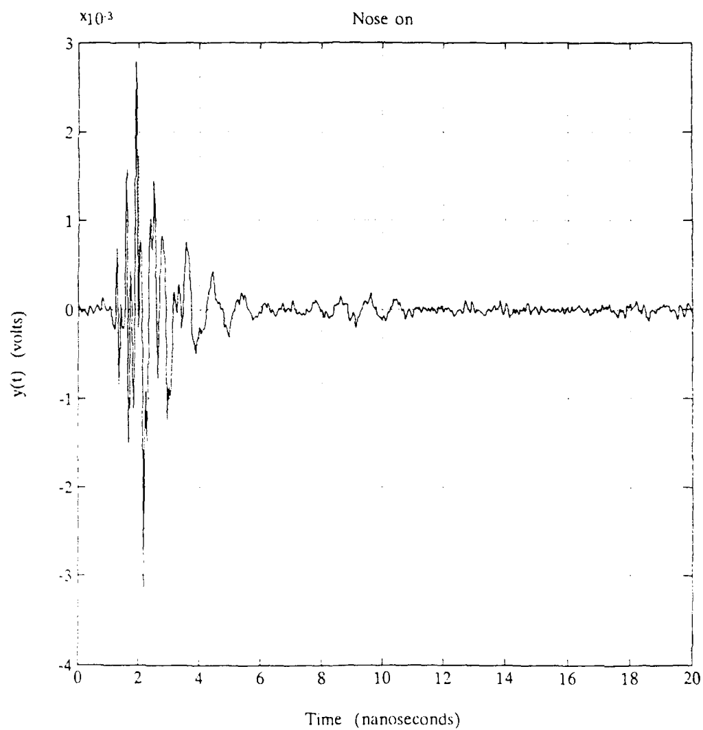
Figure 36. Target 2 Scattering, Nose on
