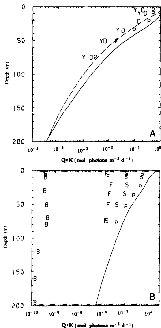
Fig. 12. A. Distribution of photons ( photons\ m^{-3} ) as a function of depth emphasizing: components of total photons ( Q_{PAR} \times K_{PAR} —solid line); photons lost to absorption of water ( Q_{PAR} \times K_w —dashed line); photons lost to total particle absorption ( Q_{PAR} \times K_p - P ); photons lost to detrital material absorption ( Q_{PAR} \times K_v - D ); photons lost to dissolved organic material absorption ( Q_{PAR} \times K_v - Y ). B. Distribution of photons ( photons\ m^{-3} ) as a function of depth partitioned into various components: total photons ( Q_{PAR} \times K_{PAR} —solid line); photons lost to absorption of phytoplankton ( Q_{PAR} \times K_p - p ); photosynthetically stored radiation (PSR—S); fluorescence (F); bioluminescence (B).
