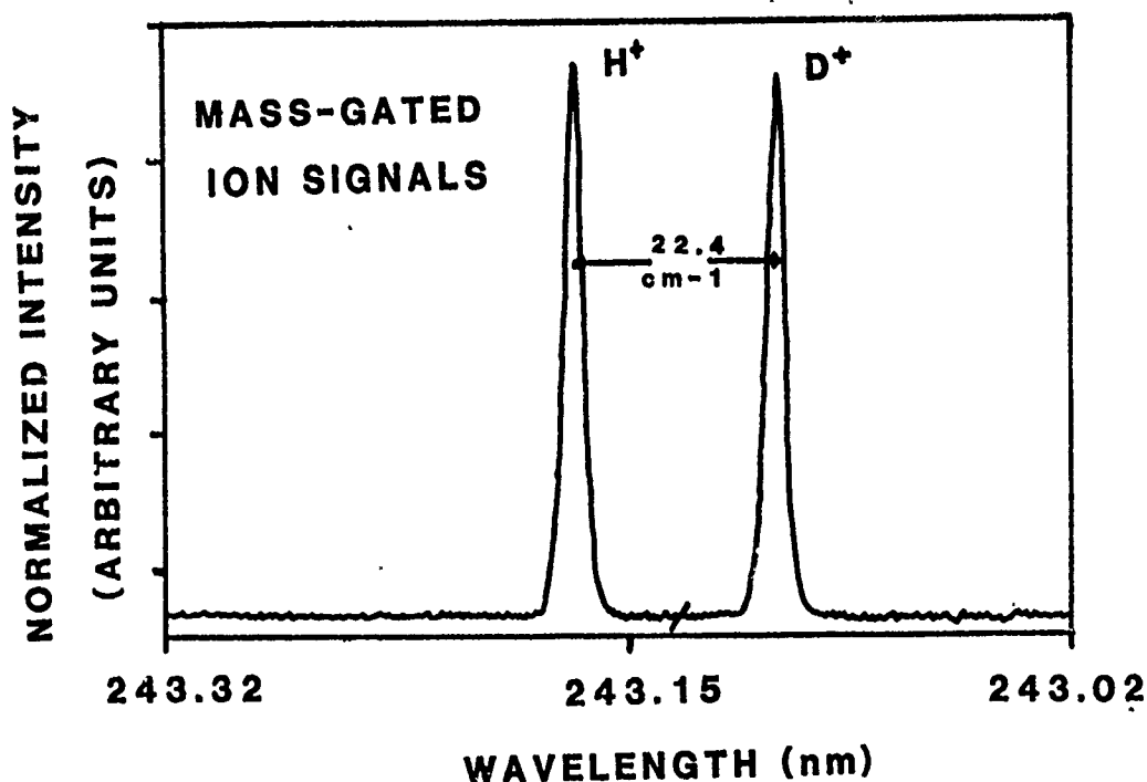
Figure 10. Mass-Gated Ion Signals (Excitation Spectrum) of H^+ and D^+ Taken in a Time-of-Flight Mass Spectrometer. An isotope of 22.4 \text{ cm}^{-1} is evident. The slash (/) indicates the wavelength position where the mass gate was shifted from H^+ to D^+ .
