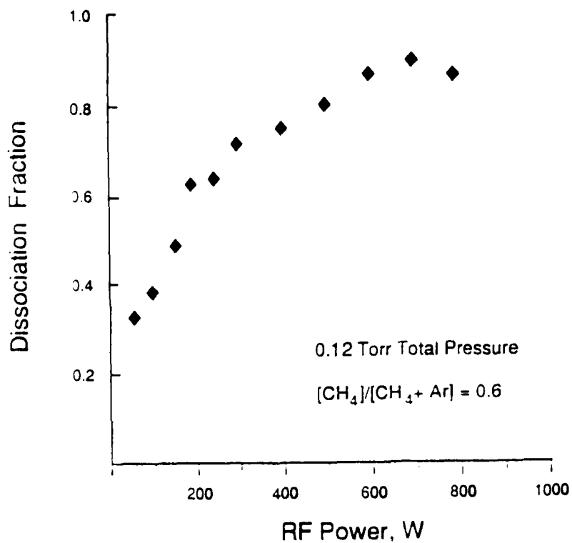
Figure 4. \text{CH}_4 Dissociation Fraction Measured by Infrared Absorption Line Intensities.
