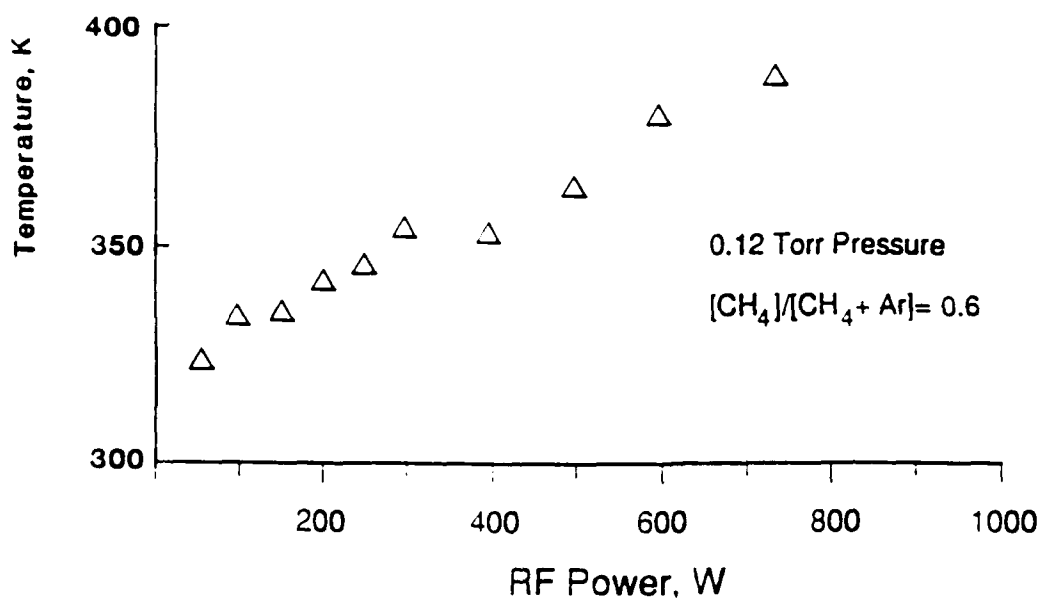
Figure 3. Methane Plasma Temperature Obtained from \text{CH}_4 Rotational Line Intensities.
