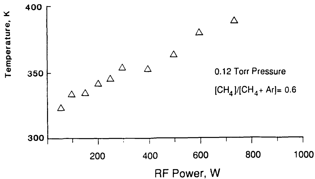
Figure 17. Methane Plasma Temperature Obtained from \text{CH}_4 Rotational Line Intensities
