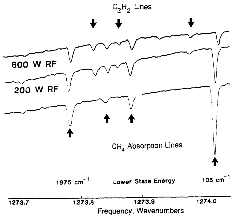
Figure 2. Infrared Spectral Region Used in CH_4 Dissociation Fraction and Temperature Measurement (Lower Trace, Plasma Off, Upper Traces, Plasma On).
