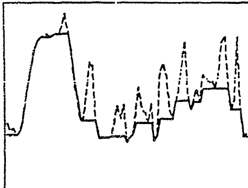
OPENING BY SET B ( |B|=5 )
