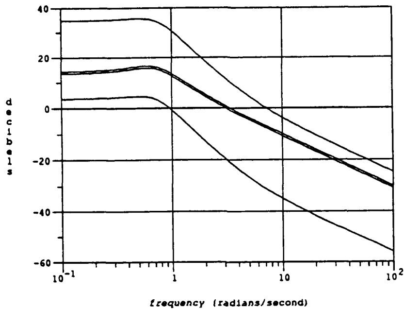
Figure 3.11: Frequency Response of the Compensator.
