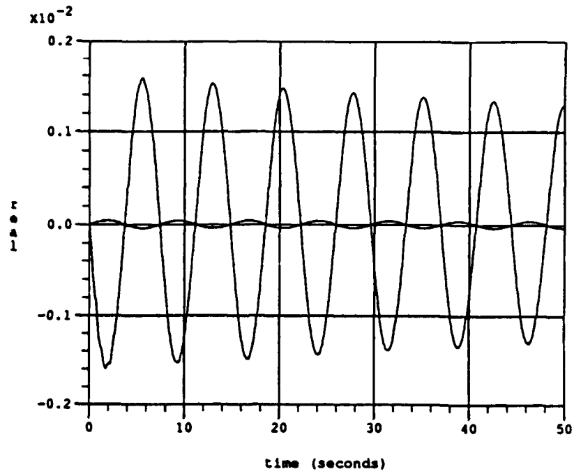
Figure 3.13: Time Response of the Open-Loop System.
