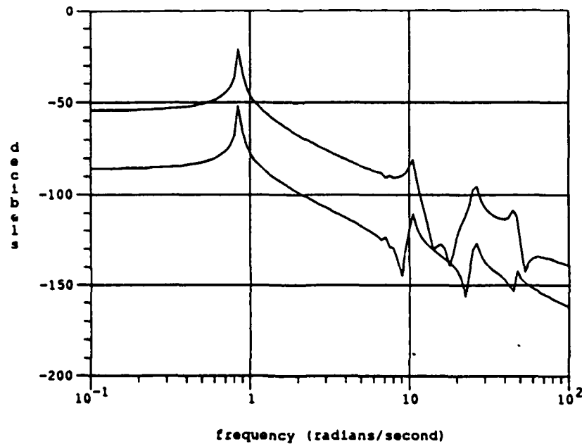
Figure 3.9: Frequency Response of the Open-Loop System.
