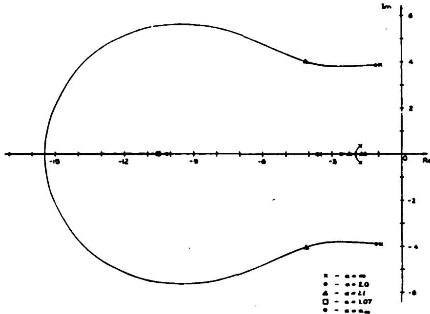
Figure 4.1: State-feedback poles for varying \alpha Example 2.
