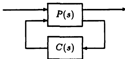
Figure 3.3: Feedback connection.
