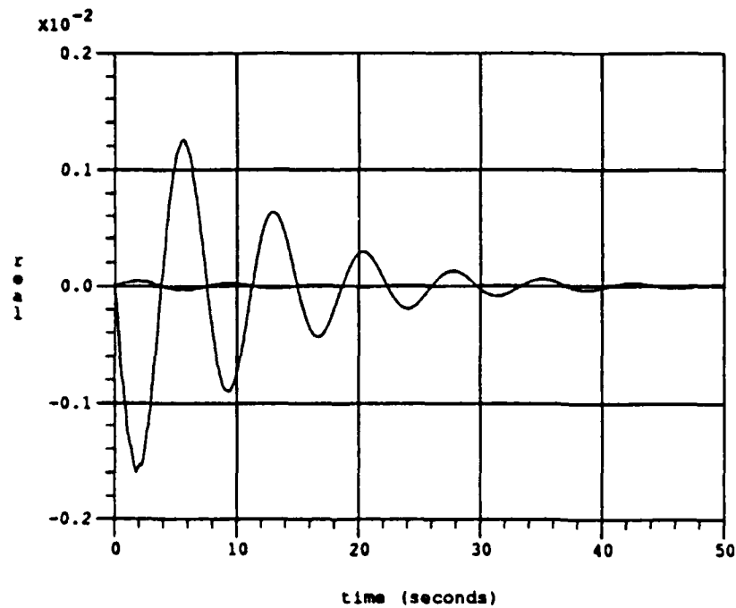
Figure 3.14: Time Response of the Closed-Loop System.
