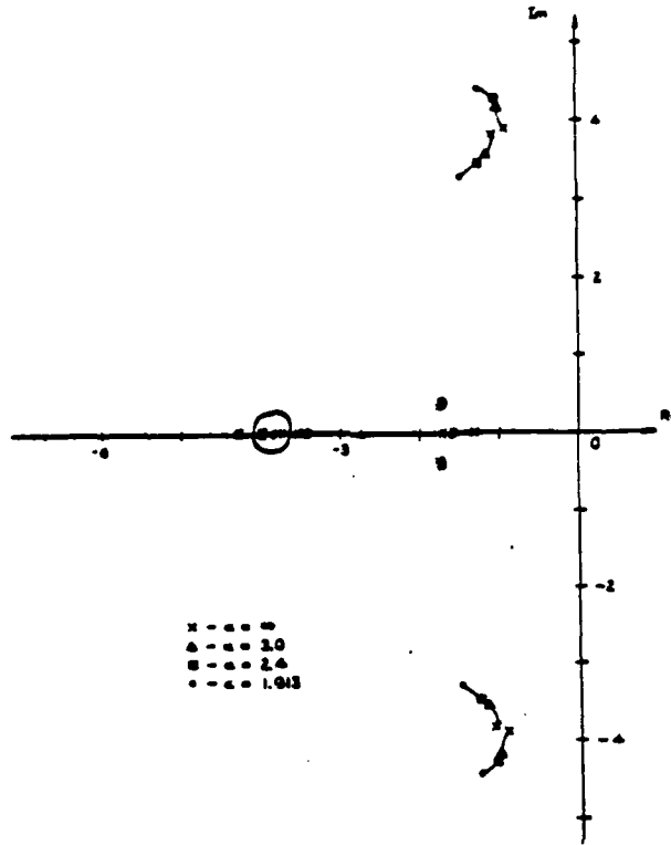
Figure 4.2: Output-feedback poles for a varying \alpha , Example 2.
