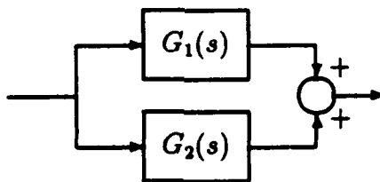
Figure 3.2: Parallel connection.
