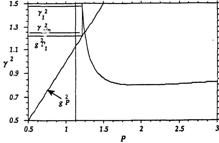
Figure 6.2: Convexity constraining condition.
