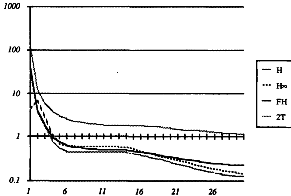
Figure 2.13: Log of various norms for the distribution of rejection problem.
