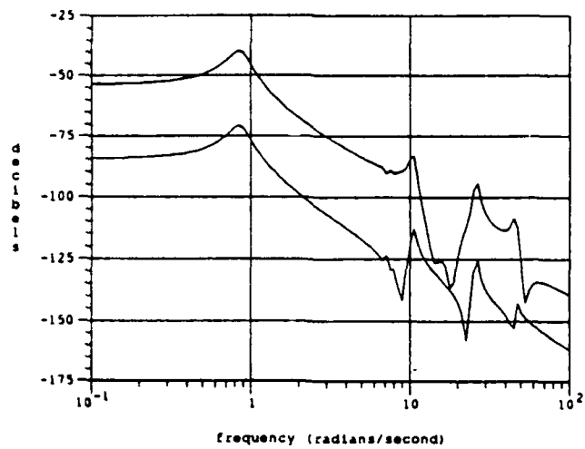
Figure 3.12: Frequency Response of the Closed-Loop System.
