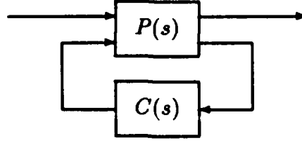
Figure 2.5: Plant with controller configuration for disturbance rejection.
