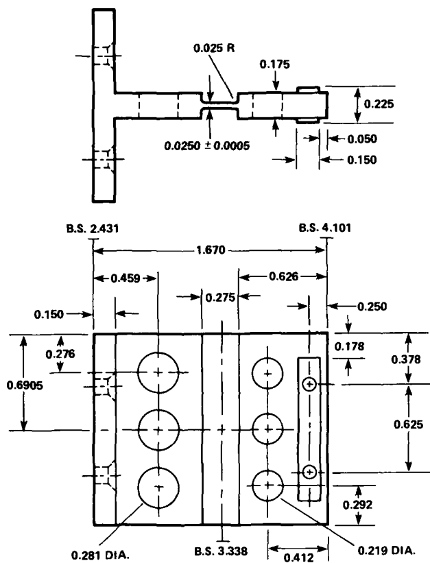
Figure 26.— Two views of lead-lag flexure.
