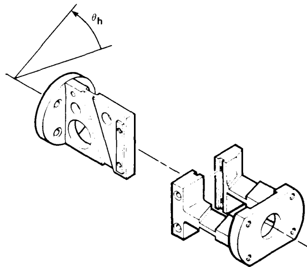
(c) Skewed flap/straight lead-lag flexures (configuration three).
