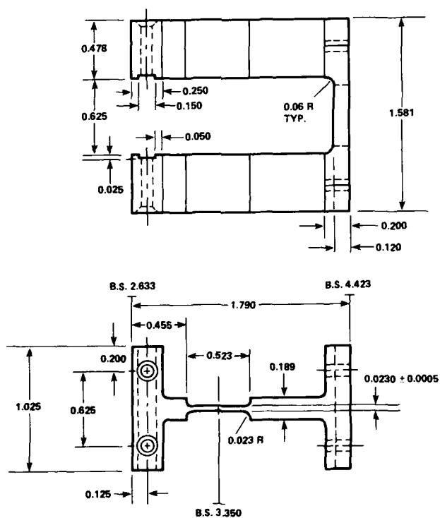
Figure 28.— Two views of flap flexure.
