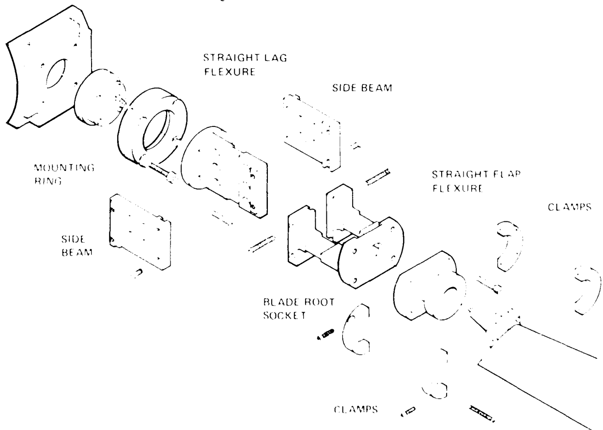
Figure 4. Rotor blade flexures.
