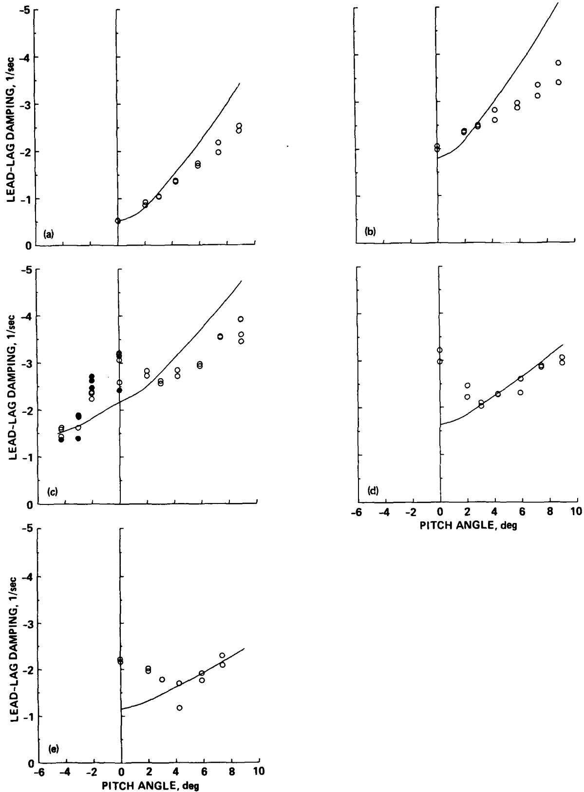
Figure 21.— Lead-lag damping as a function of blade pitch angle for the skewed flap/skewed lead-lag flexure (configuration four); \bar{\omega}_\zeta = 0.70 . Excitation at \Omega - \omega_\zeta shown by solid symbols. (a) \theta_h = 0^\circ , (b) \theta_h = 18^\circ , (c) \theta_h = 36^\circ , (d) \theta_h = 51^\circ , (e) \theta_h = 60^\circ .
