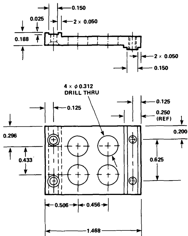
Figure 27.— Two views of flexure side beam.
