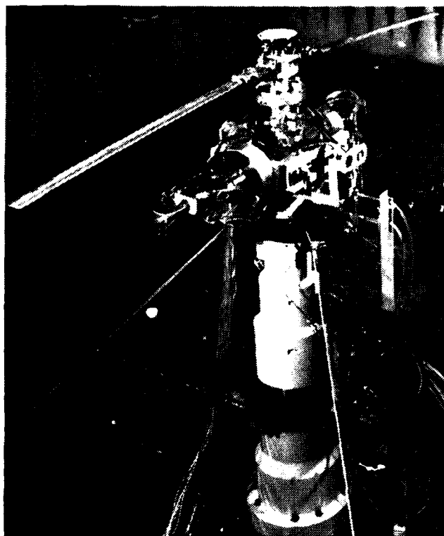
Figure 35.— Two-bladed rotor model used during second experiment.
