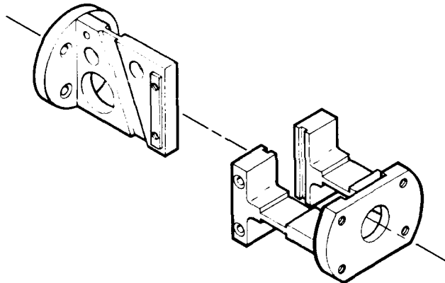
(b) Straight flap/skewed lead-lag flexures (configuration two).
