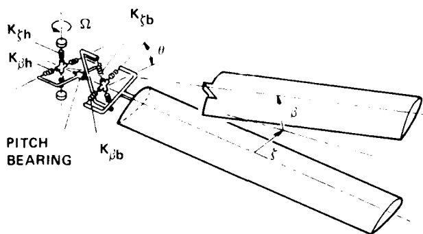
Figure 2.— Representation of hingeless rotor blade with spring-restrained, centrally hinged, rigid blade. (For clarity, blade springs are shown offset from axis of rotation.)
