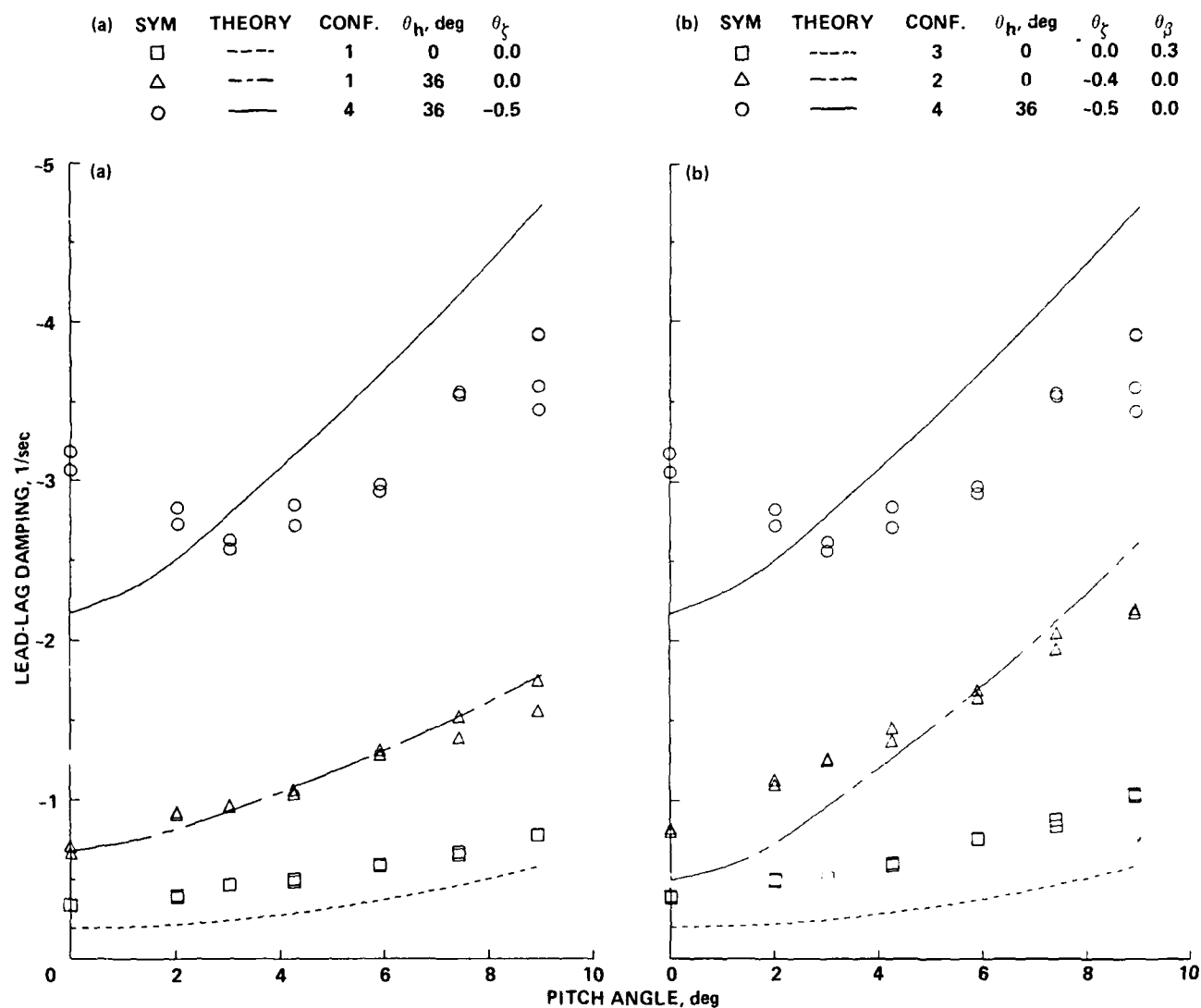
Figure 23.— Lead-lag damping as a function of blade pitch angle, \bar{\omega}_\zeta = 0.70 . (a) Comparison of combined pitch-lag and flap-lag coupling (configuration four), flap-lag coupling alone (configuration one with flexure inclination of 36°), and no coupling (configuration one with zero flexure inclination). (b) Comparison of combined pitch-lag coupling (configuration four), pitch-lag coupling alone (configuration two), and pitch-flap coupling alone (configuration three).
