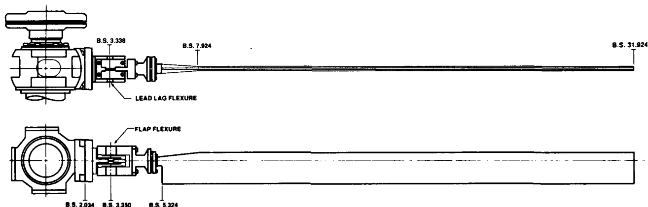
Figure 25.— Two views of rotor hub and blade.
