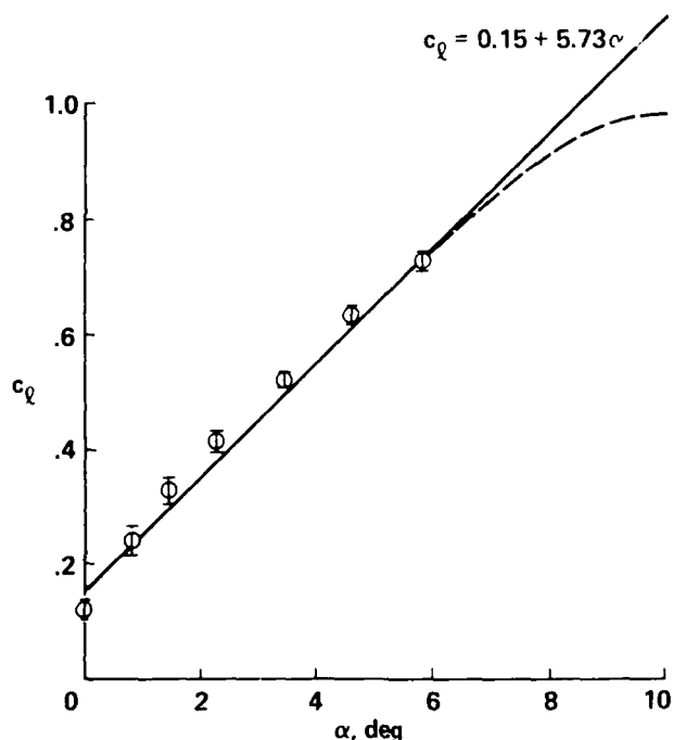
Figure 33.— Section lift coefficient derived from steady bending moment data for configuration four, Re \approx 130,000 . Dashed curve is from reference 13, Re \approx 250,000 .
