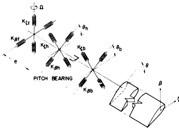
Figure 24.— Three-spring model of blade flexibility.
