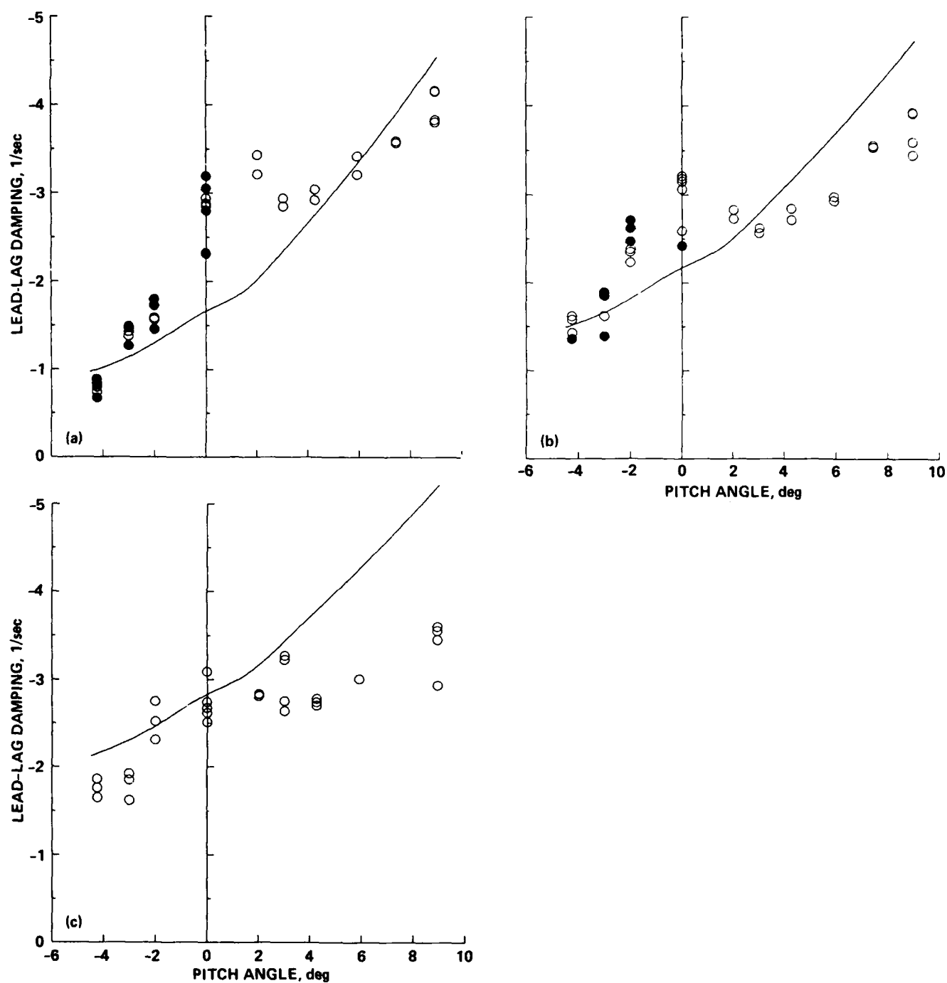
Figure 22.— Lead-lag damping as a function of blade pitch angle for the skewed flap/skewed lead-lag flexure (configuration four); \theta_h = 36^\circ . Excitation at \Omega - \omega_\zeta shown by solid symbols. (a) \bar{\omega}_\zeta = 0.60 , (b) \bar{\omega}_\zeta = 0.70 , (c) \bar{\omega}_\zeta = 0.80 .
