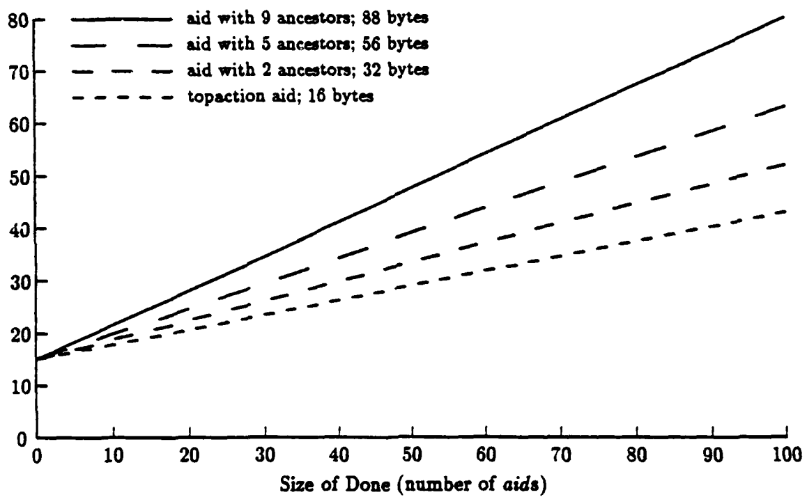
Figure 7.1: Cost of Piggybacking Done
