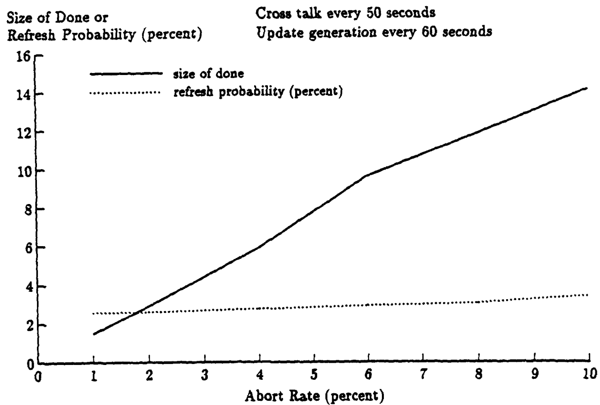
Figure 7.20: Performance for different abort rates — two subsystems
