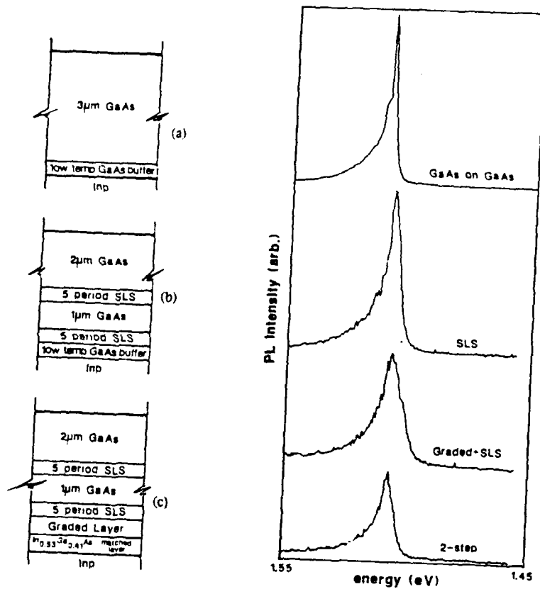
Fig.1 Schematics of different buffer structures: (a) Low temperature grown GaAs buffer layer; (b) 2 sets of \text{In}_{0.05}\text{Ga}_{0.95}\text{As}/\text{GaAs} SLS; (c) Transitional graded \text{In}_{0.33}\text{Ga}_{0.67}\text{As} layer plus 2 sets of \text{In}_{0.05}\text{Ga}_{0.95}\text{As}/\text{GaAs} SLS.
