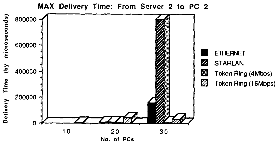
Figure A-14. MAX Delivery Time for Transaction Class 2 with Two Server: From Server to PC
