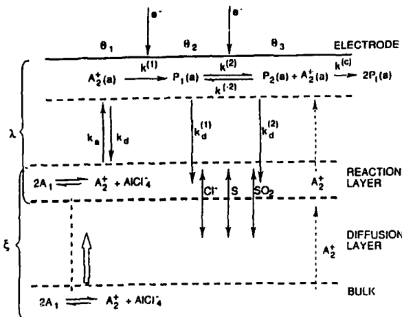
Figure 4. Summary of SOCl 2 reduction path.
