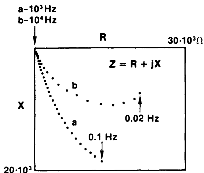
Fig 5 Nyquist Plot. Electrode - Glassy Carbon; Area - 0.316 \text{ cm}^2 . Electrolyte - 1\text{M LiAlCl}_4 in \text{SOCl}_2 for Curve a 1\text{M LiAlCl}_4 in \text{SOCl}_2 saturated with Fe-phthalocyanine for Curve b.
