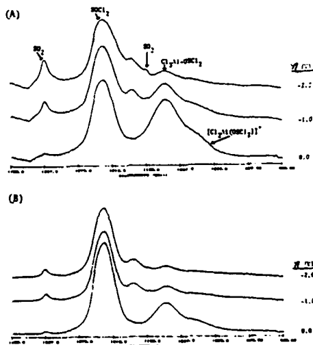
Fig. 2. The 900 to 1400 \text{cm}^{-1} spectral region of the metal/electrolyte interphase.
