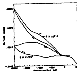
Fig. 1 Cyclic Voltammograms of 2.0M and 3.0M \text{AlCl}_3 in \text{SOCl}_2 on Pt at 50\text{ mV s}^{-1} .
