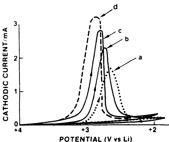
Fig. 4. Cyclic voltammograms on glassy carbon: scan rate—50 mV s -1 , electrode area—0.314 cm 2 , and electrolyte—1.0M LiAlCl 4 in SOCl 2 . Curve a (no additives), curve b (saturated with Cu-Pc), curve c (saturated with Fe-Pc), and curve d (saturated with Co-Pc).
