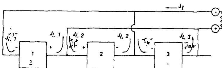
Fig. 2 Multimodule battery representation.
