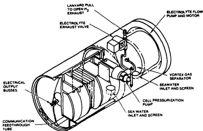
Fig. 1 Multimodule battery assembly including accessories
