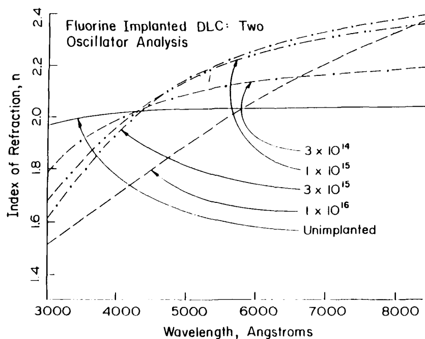
Figure 3 Index of Refraction for Ion Beam Deposited Samples after F Implantation at the Fluences Indicated
