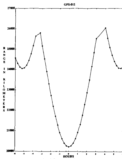
Fig. 10. Range variation for GPS-012 orbit
