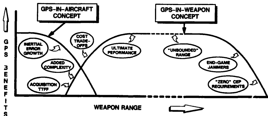
Figure 10. GPS-in-Aircraft &amp; GPS-in-Weapon Concepts And Relative Benefit To Weapon Guidance
