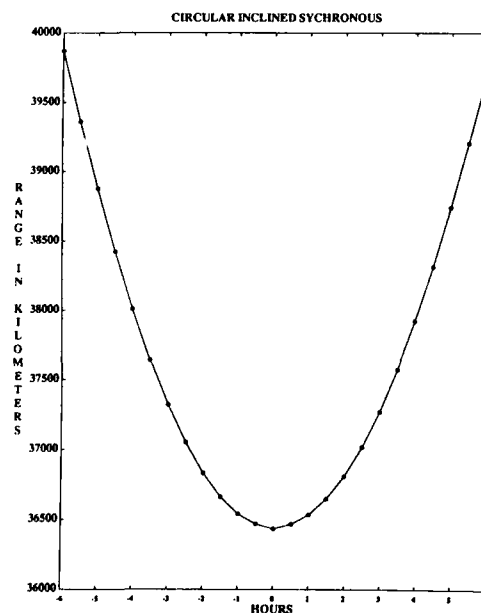
Fig. 6. Range variation for CIS orbit
