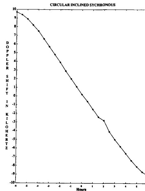
Fig. 7. Doppler shift with CIS orbit
