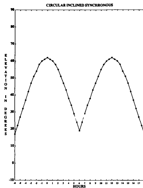
Fig. 5. Elevation variation with two CIS orbit satellites
