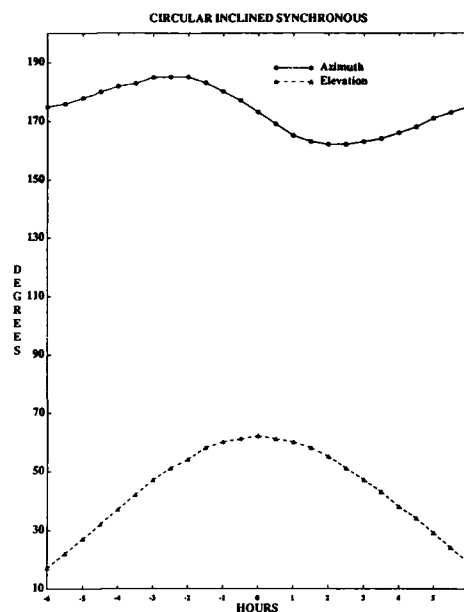
Fig. 4. Azimuth and elevation variation for CIS orbit
