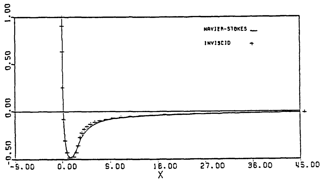
Figure 8. Surface pressure coefficient C_p ; AR = 3 , Re_L = 2400 .
