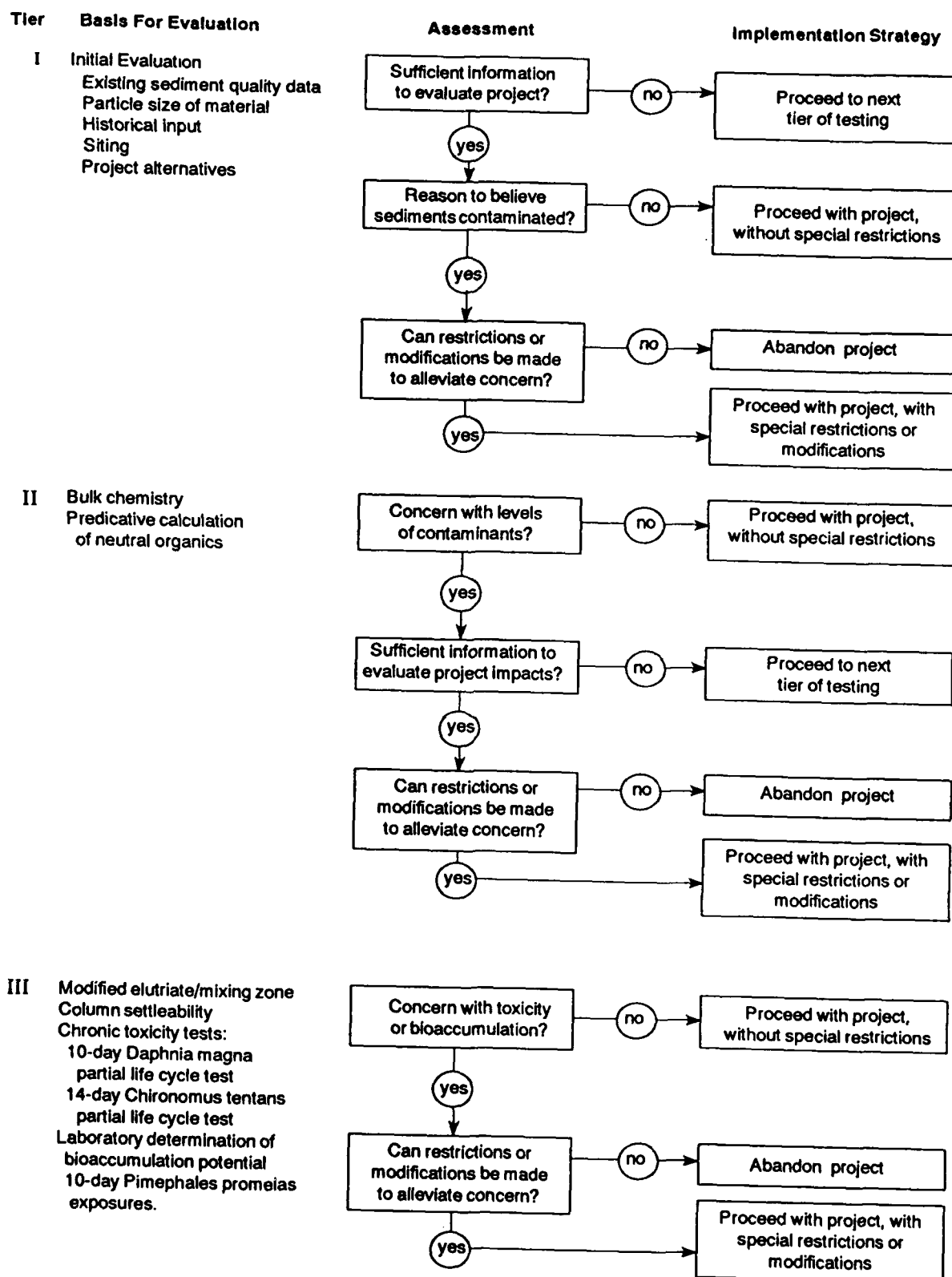
Figure 1. Tiered Sediment Testing Protocol for HREP's
