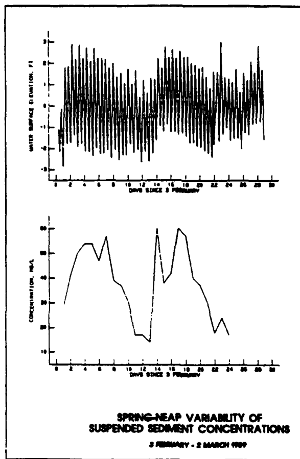
Figure 4. Spring - neap variability of tides and the effect on the suspended sediment concentrations.
