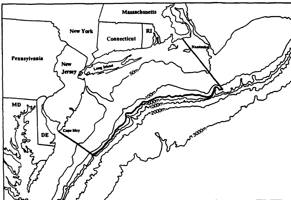
Figure 1. Proposed boundaries for New York Bight models
