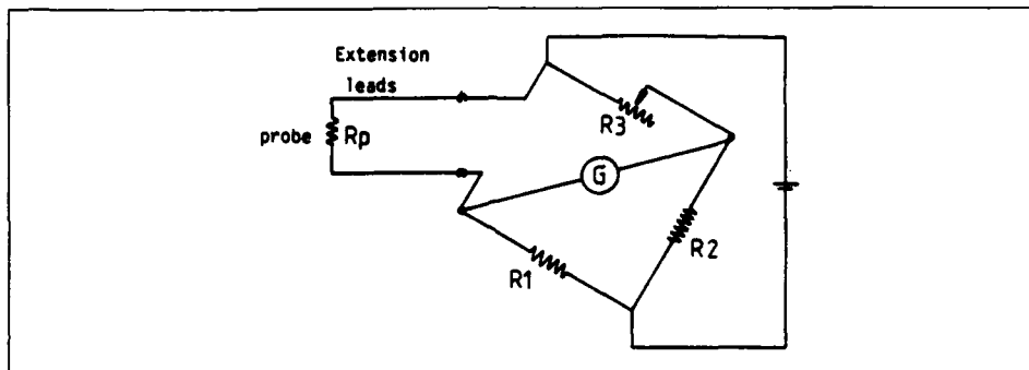
Fig. 6.3-3 Resistance measurement with Wheatstone bridge circuit: 2-wires system
