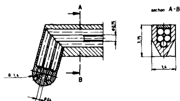
SENSOR DETAIL
