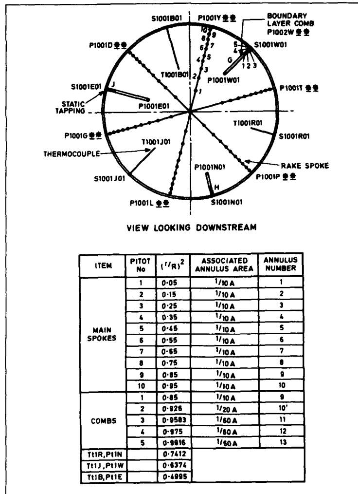
Fig. 2.4-3 Inlet duct instrumentation at engine inlet plane
