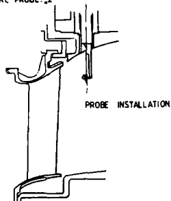
SENSOR DETAIL
