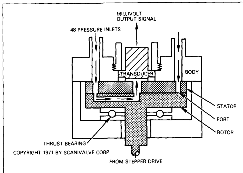
Fig. 5.3-6 Pressure scanner module
