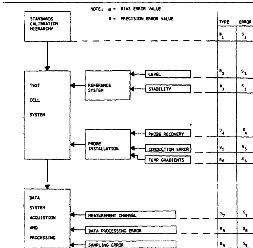
TEMPERATURE MEASUREMENT ERROR SOURCE DIAGRAM
