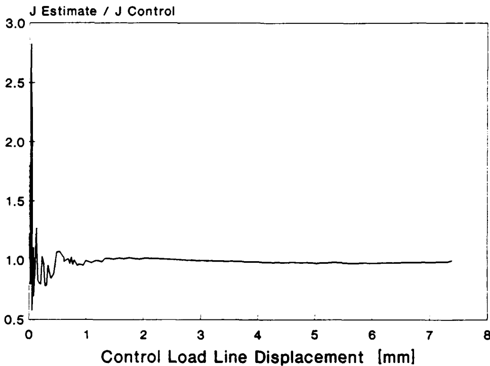
Figure 16: A comparison of applied J calculated from the reference load and load line displacement estimates with that calculated from load and load line displacement estimated using the candidate procedures for the low hardening steel.
