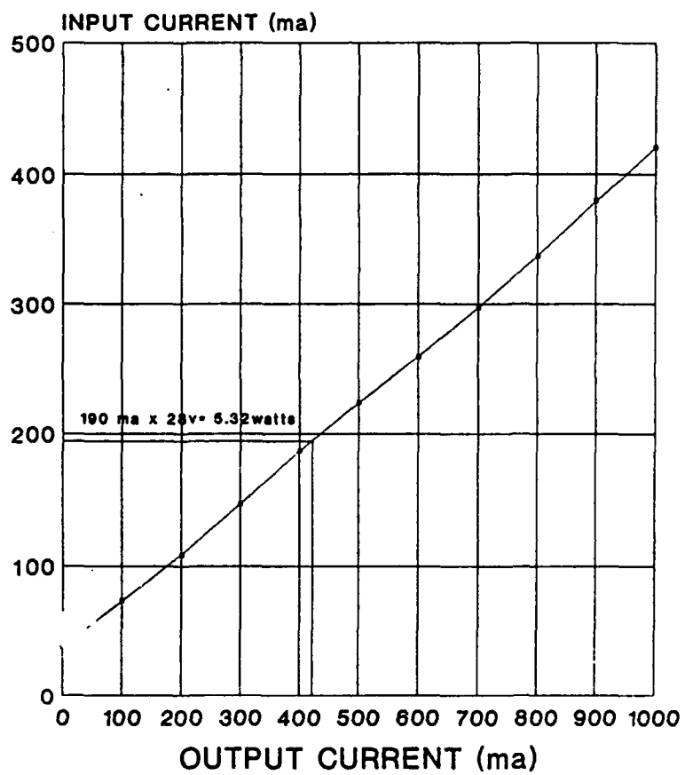
Figure 3.4 Bus Power Required to Support 5 v Power Supply
