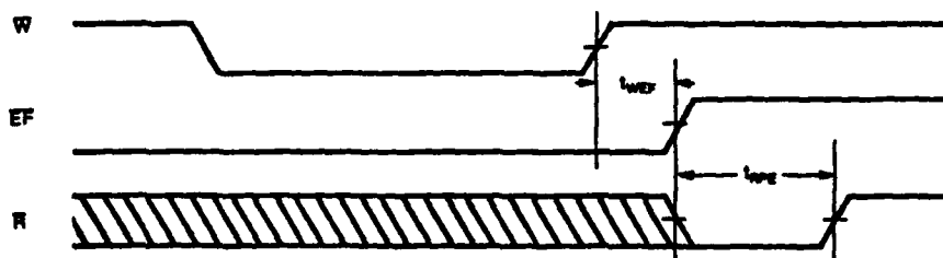
Figure 7. Empty Flag Timing
