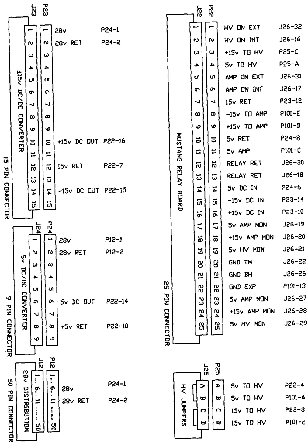
Figure 4.2b Support Components Required to MUSTANG [Ref. 9]
