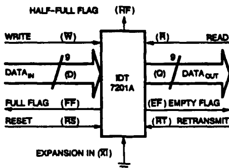
Figure 12. Block Diagram of Single 512x9 FIFO
