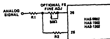
Figure 3. Full Scale Trim
