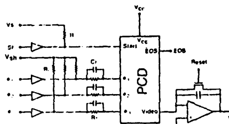
Figure 7: Driving and amplifier circuit
