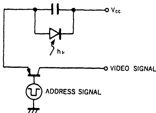
Figure 2.18 Switch Section Equivalent Circuit [Ref. 5:p. 1]
