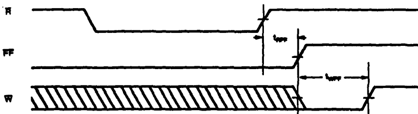
Figure 8. Full Flag Timing
