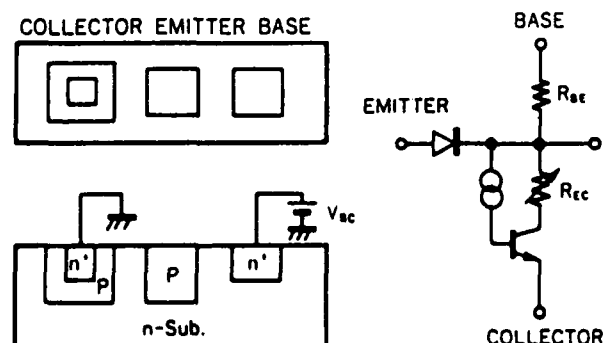
Figure 2.16 HCDT Equivalent Circuit [Ref. 5:p. 1]
