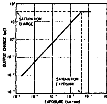
Figure 4: Output charge vs. exposure
