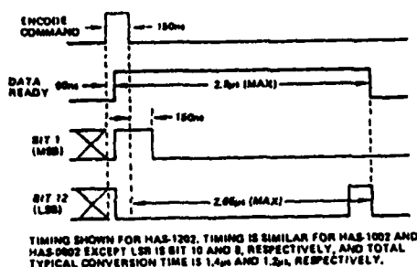
Figure 1. Timing Diagram (Typical)
