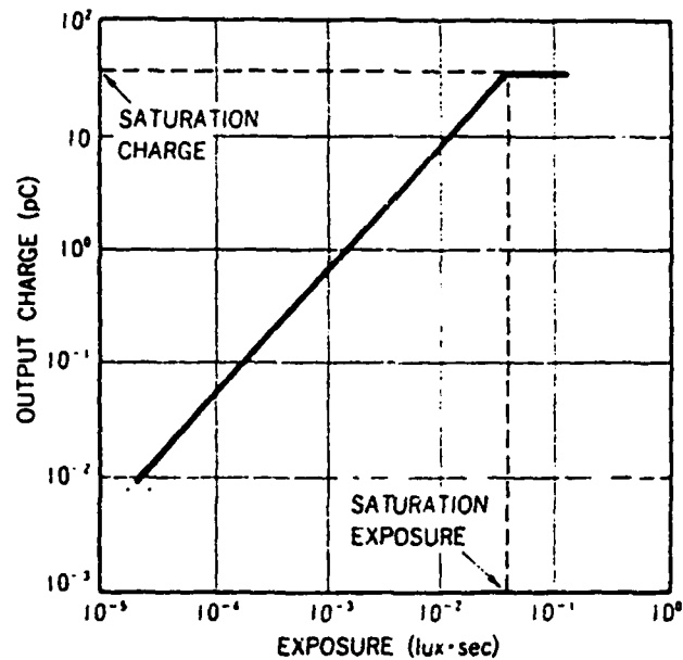
Figure 2.10 Image Sensor Photoelectric Conversion Characteristics [Ref. 5:p. 8]
