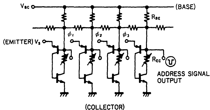
Figure 2.15 PCD Shift Register Equivalent Circuit [Ref. 5:p. 1]
