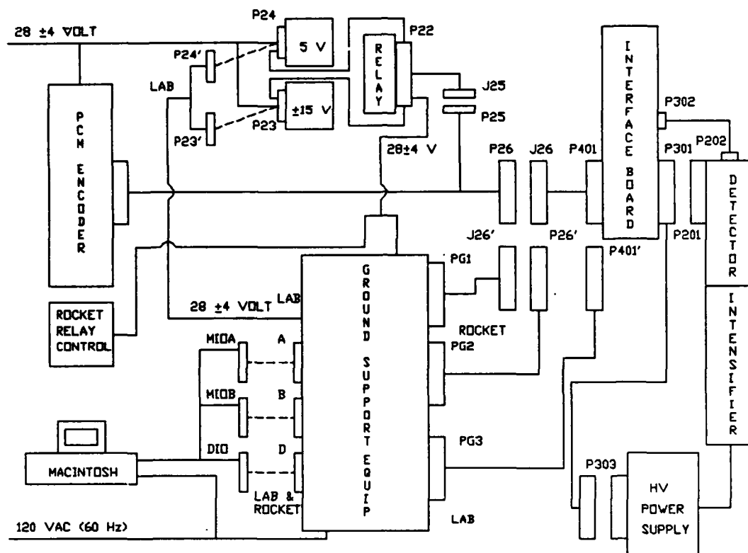
Figure 4.1 Block Diagram of GSE MUSTANG Interface
