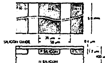
Figure 2: Sensor geometry
