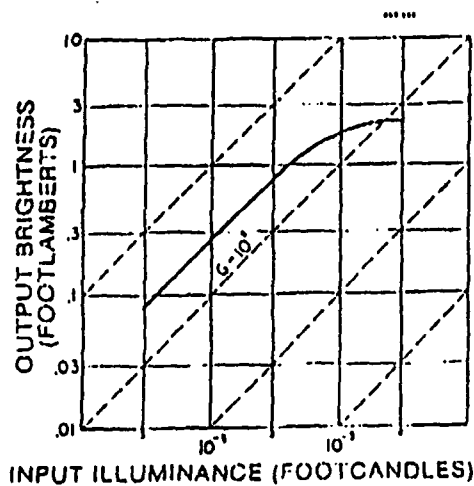
TYPICAL SATURATION CURVE OF PROXIMITY FOCUSED MICROCHANNEL WAFER TUBE
