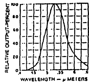
SPECTRAL OUTPUT P-20 PHOSPHOR
