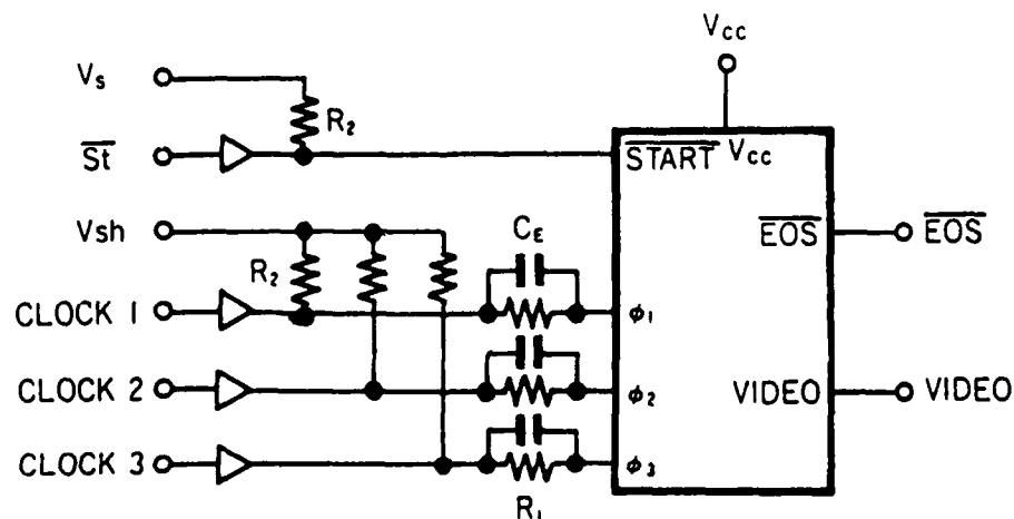
Figure 2.17 Clock Driver Circuit [Ref. 5:p. 2]
