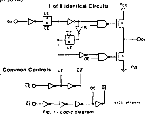
Fig. 1 - Logic diagram.
