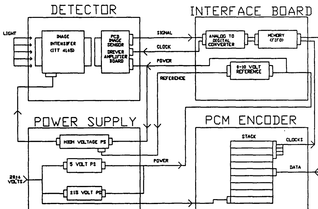
Figure 2.1 Block Diagram of Mustang Subsystems
