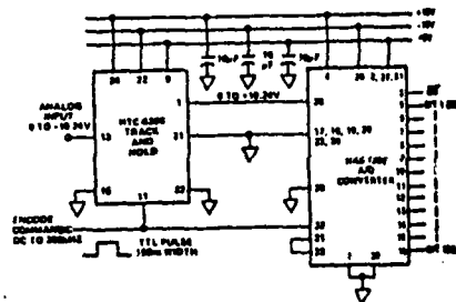
Figure 4. DC to 350kHz, 12-Bit, A/D Conversion System
