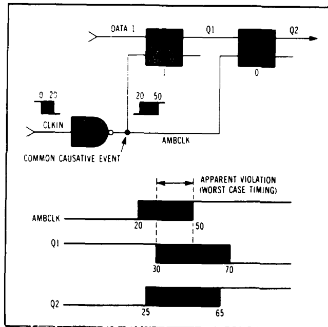
Fig I3 — Shared delays in reconverging signals cause a condition called "common ambiguity" during worst-case timing analysis. In this example, it is not clear from the AMBCLK and Q1 waveforms whether a 0 or 1 will be locked at flip-flop 0. But a look at the circuit's topology reveals that 30 ns of ambiguity stems from a common source. By removing this ambiguity, Teradyne's Lasar simulator finds that stable data is being clocked into the flip-flop, yielding the waveform shown for Q2.
