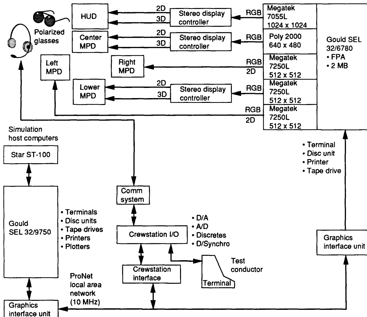
Figure 3.1-1. Schematic Diagram of Major Simulation Elements
