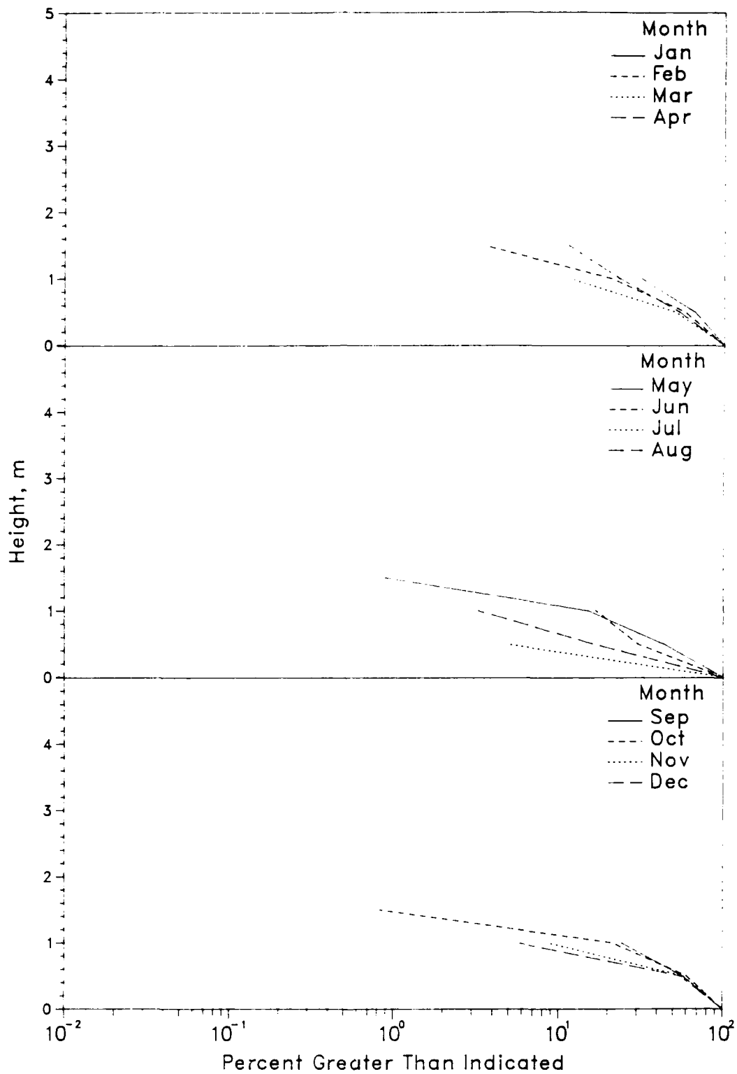
Figure E3. 1988 monthly wave height distributions for Gage 645
