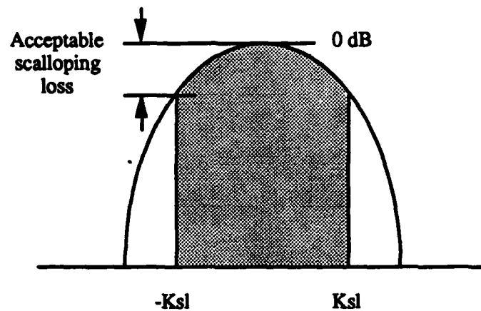
Figure 3.14 Scalloping loss limit on mainlobe of beampattern.
