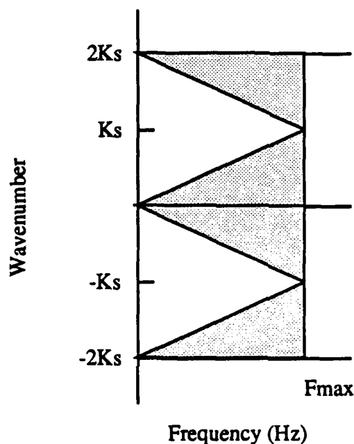
Figure 3.9 Wavenumber spectrum.
