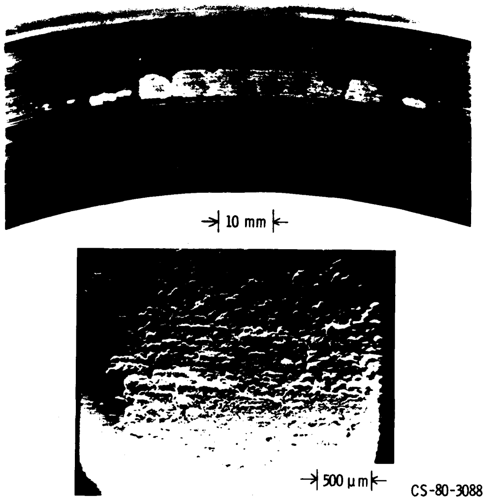
Fig.3 Peeling failure on cup raceway surface after 569 hours with standard design bearing run at 12,500 rpm
