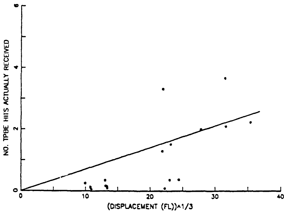
Figure 3. Torpedo Damaged Platforms Plotted Over Model Line
