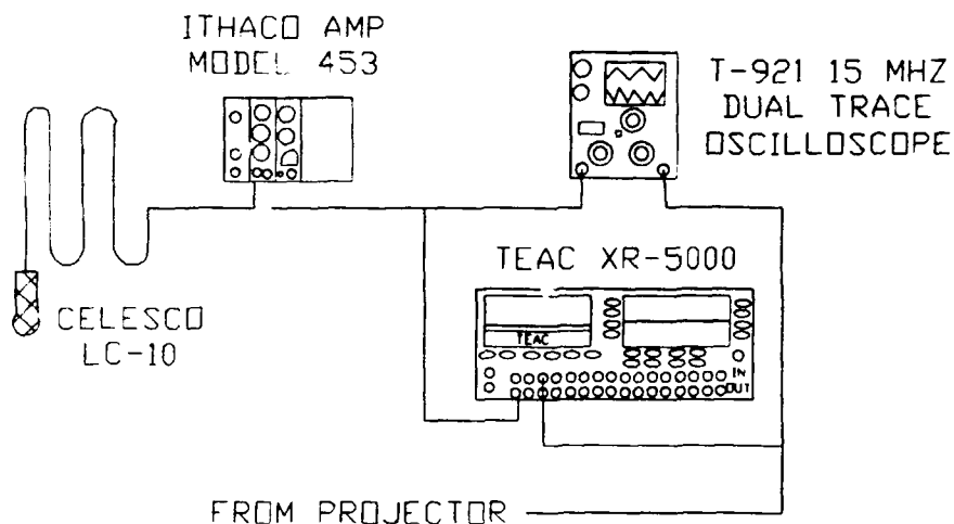
Figure 3.4 Hydrophone schematic
