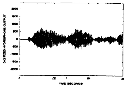
Hydrophone 8 without scattering plate
