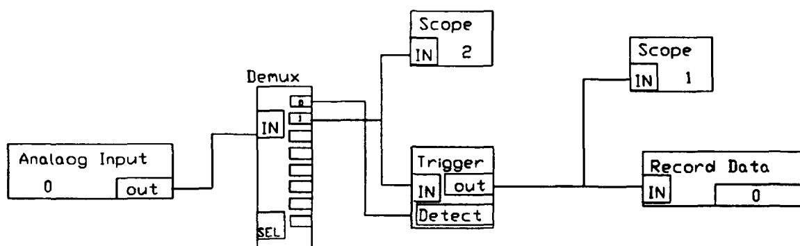
Figure 3.7 Lab Workbench A/D conversion virtual instrument.
