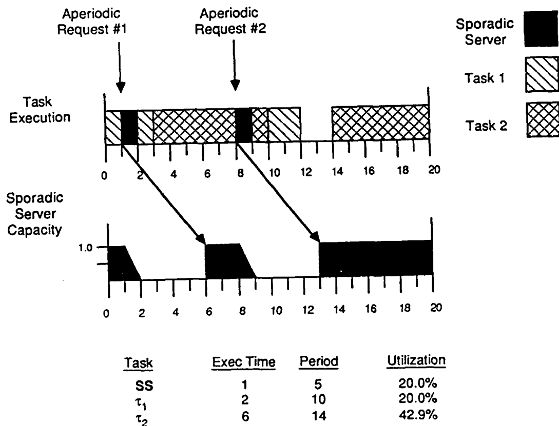
Figure 1: High Priority Sporadic Server Example
