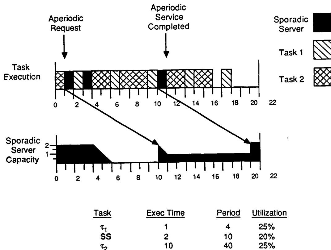
Figure 4: Exhausted Sporadic Server Replenishment
