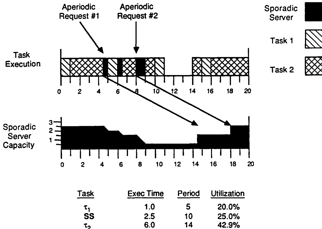
Figure 3: Medium Priority Sporadic Server Example
