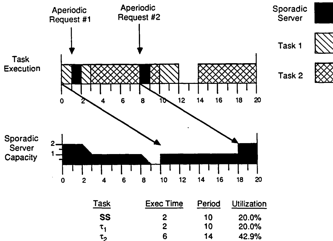
Figure 2: Equal Priority Sporadic Server Example
